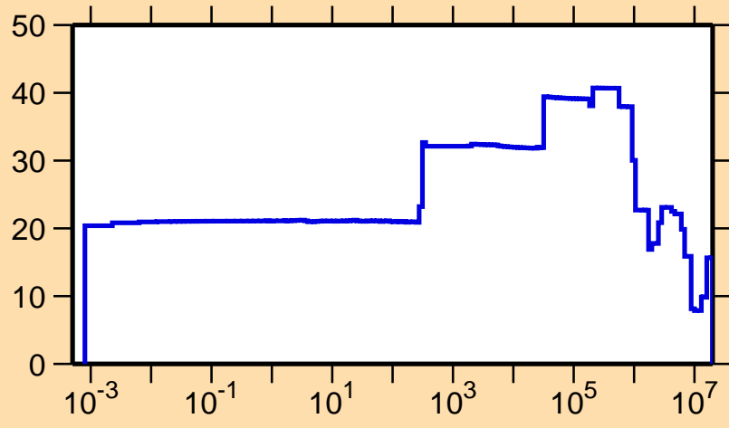
\Delta\sigma/\sigma vs. E for ^{258}\text{Md}(n,el.)
