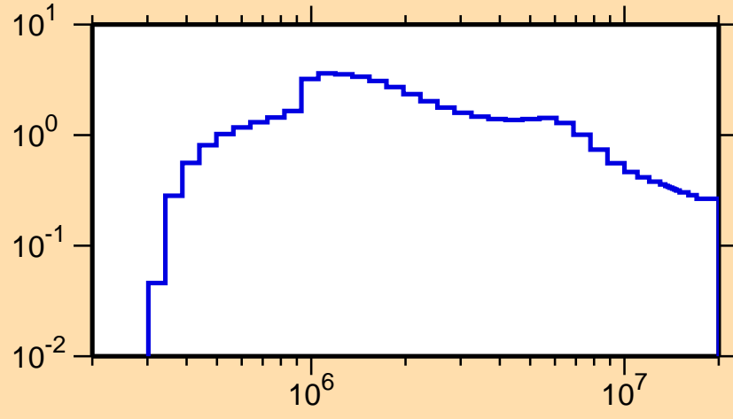
\sigma vs. E for ^{258}\text{Md}(n,\text{inel.})
