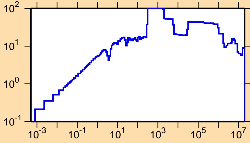
\Delta\sigma/\sigma vs. E for ^{258}\text{Md}(n,tot.)
