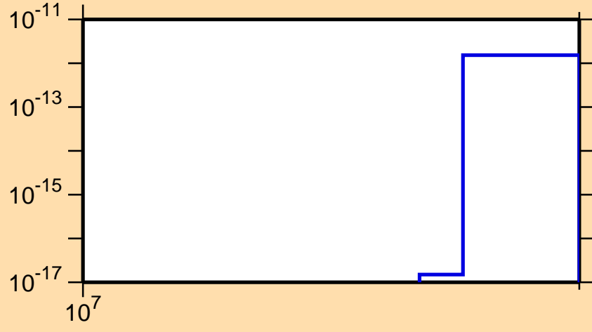
\sigma vs. E for ^{258}\text{Md} (mt 42)
