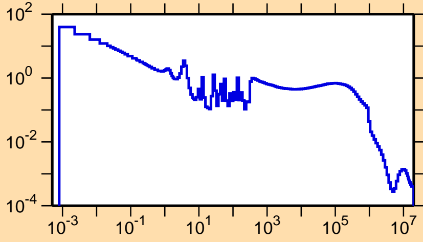
\sigma vs. E for ^{258}\text{Md}(n,\gamma)
