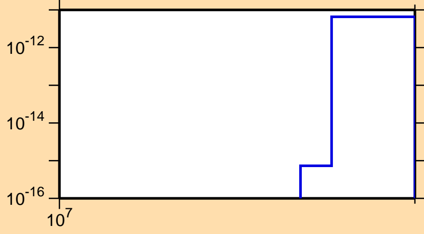
\sigma vs. E for ^{258}\text{Md} (mt 11)
