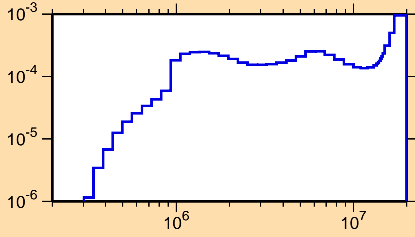
\sigma vs. E for ^{258}\text{Md}(n,n\alpha)
