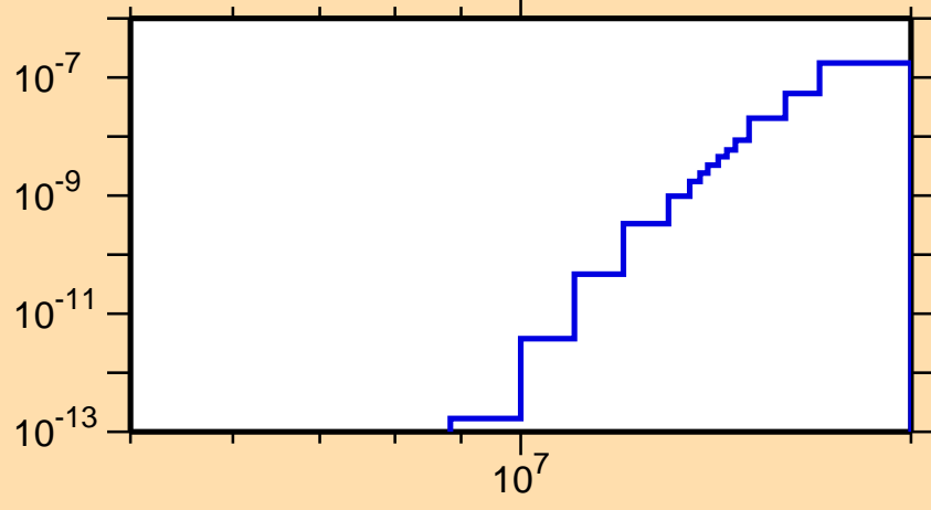
\sigma vs. E for ^{258}\text{Md}(\text{mt } 45)
