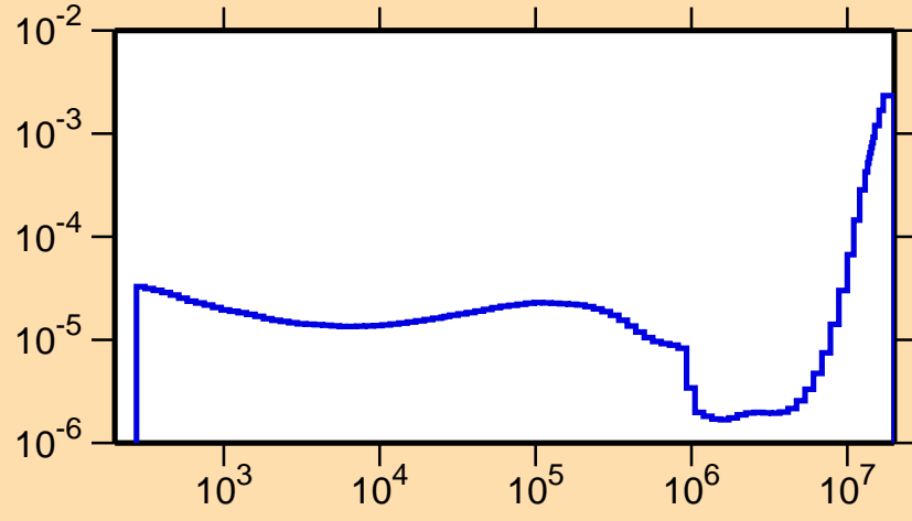
\sigma vs. E for ^{258}\text{Md}(n,\alpha)
