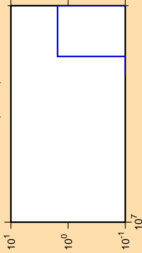
\Delta\sigma/\sigma vs. E for ^{258}\text{Md} (mt 42)
