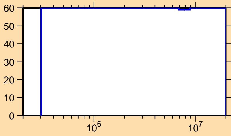
\Delta\sigma/\sigma vs. E for ^{258}\text{Md}(n,n\text{cont.})
