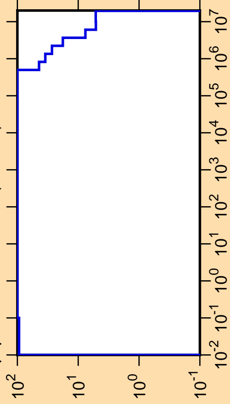
\Delta\mu/\mu vs. E for ^{258}\text{Md}(\text{mt251})
