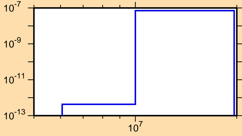
\sigma vs. E for ^{258}\text{Md}(\text{mt117})
