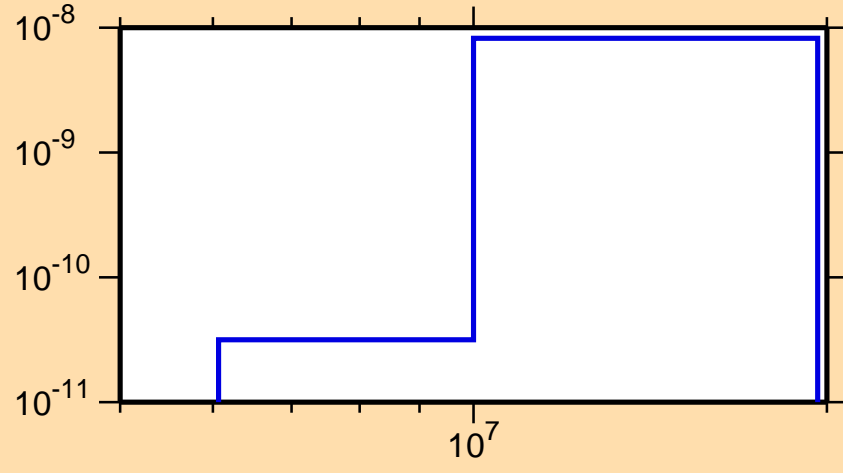
\sigma vs. E for ^{258}\text{Md}(n,p\alpha)
