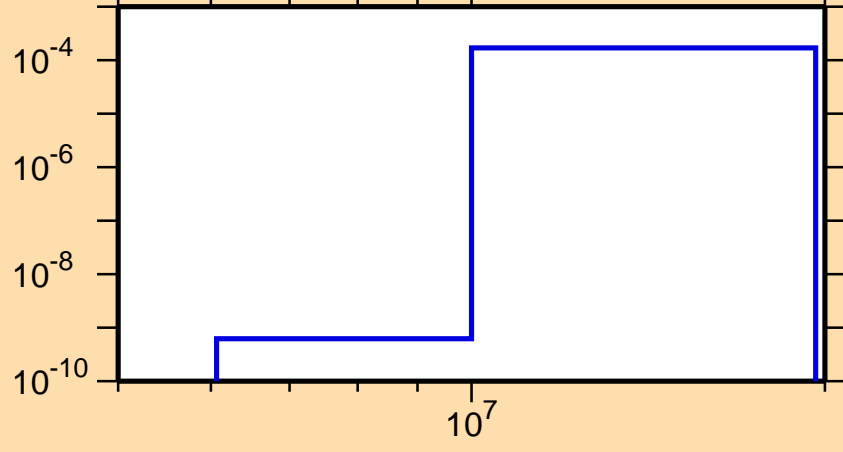
\sigma vs. E for ^{258}\text{Md}(n,t)
