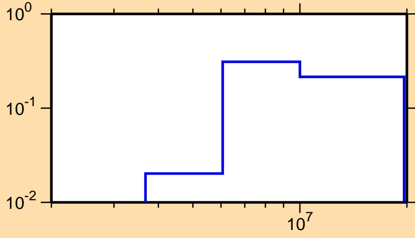
\sigma vs. E for ^{258}\text{Md}(n,2n\alpha)
