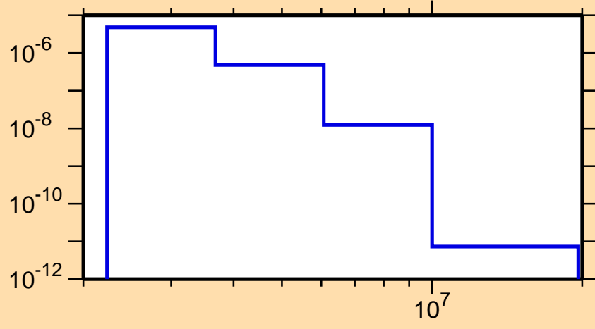
\sigma vs. E for ^{258}\text{Md}(n,n_4)
