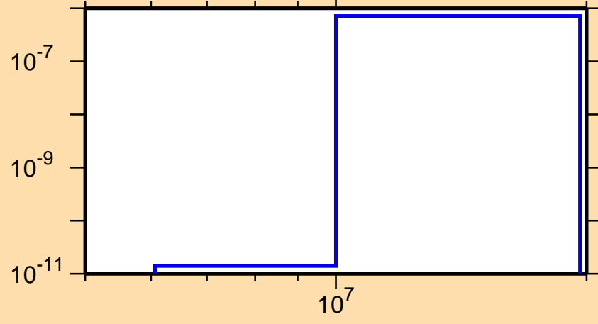
\sigma vs. E for ^{258}\text{Md}(\text{mt117})
