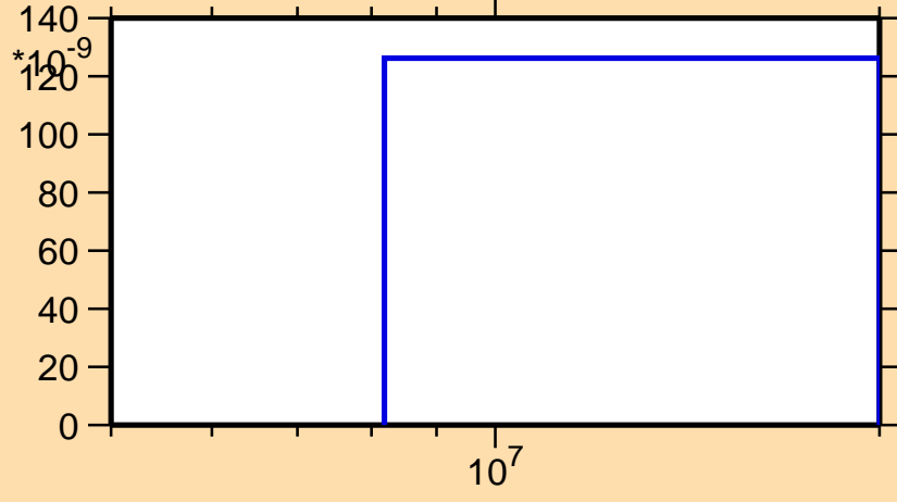
\sigma vs. E for ^{258}\text{Md}(\text{mt } 45)
