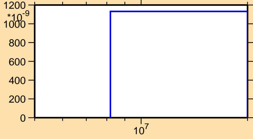
\sigma vs. E for ^{258}\text{Md}(n,nd)
