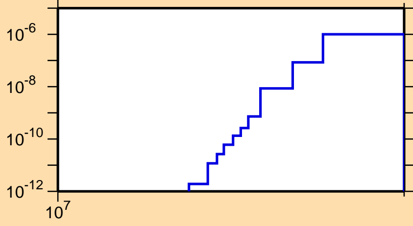
\sigma vs. E for ^{259}\text{Md}(n,\text{nd})
