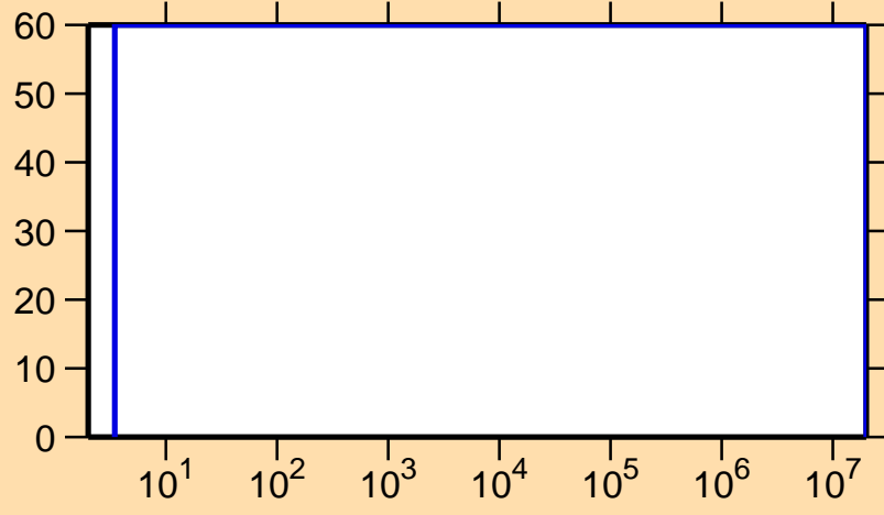
\Delta\sigma/\sigma vs. E for ^{259}\text{Md}(n,\gamma)
