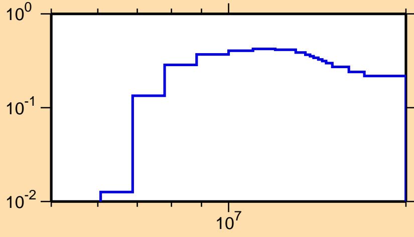
\sigma vs. E for ^{259}\text{Md}(n,2n)
