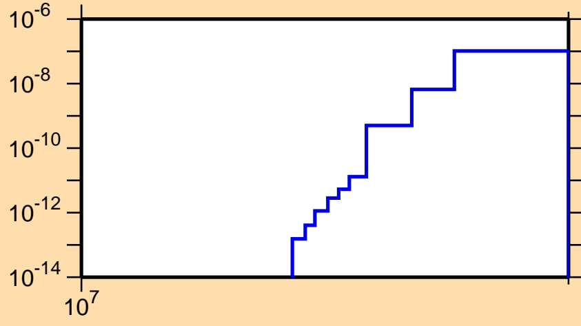
\sigma vs. E for ^{259}\text{Md}(n,2np)
