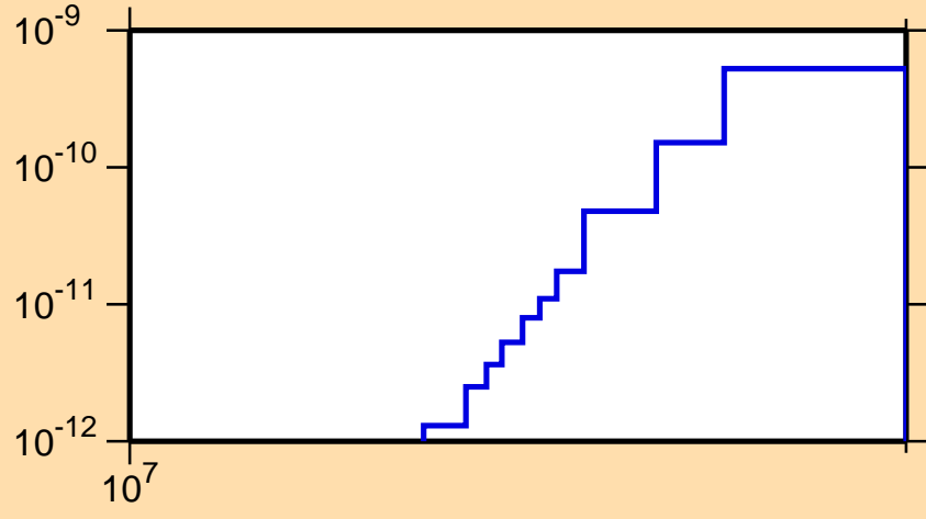
\sigma vs. E for ^{259}\text{Md} (mt 45)
