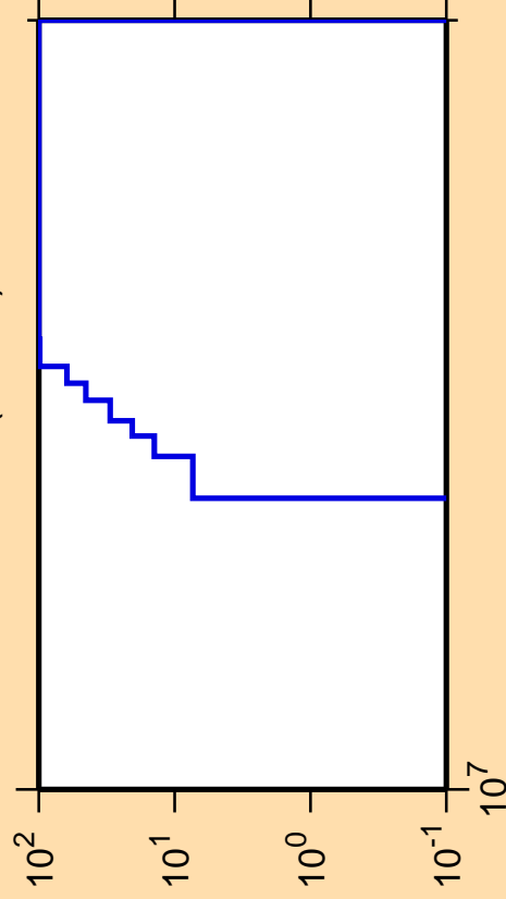
\Delta\sigma/\sigma vs. E for ^{259}\text{Md} (mt 45)
