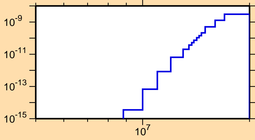
\sigma vs. E for ^{259}\text{Md}(\text{mt117})
