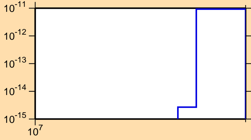
\sigma vs. E for ^{259}\text{Md} (mt 11)
