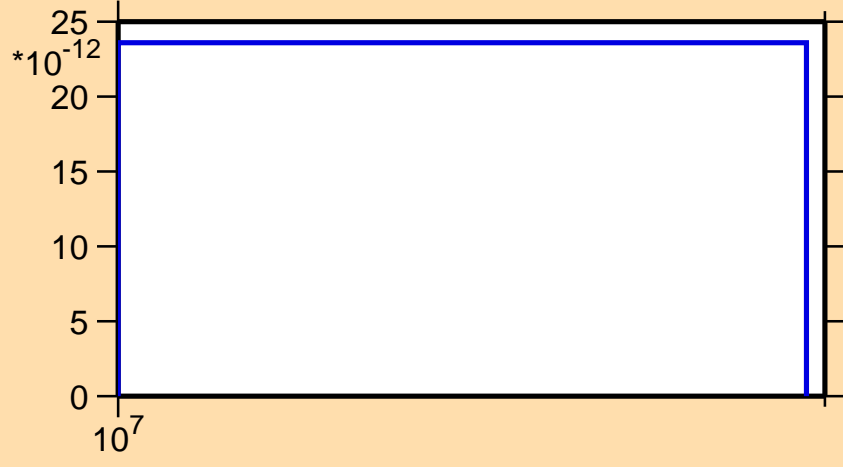
\sigma vs. E for ^{259}\text{Md} (mt 45)
