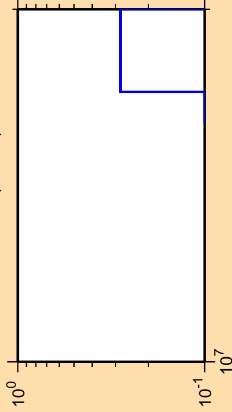
\Delta\sigma/\sigma vs. E for ^{260}\text{Md} (mt 42)
