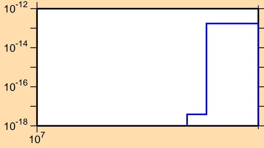
\sigma vs. E for ^{260}\text{Md} (mt 42)
