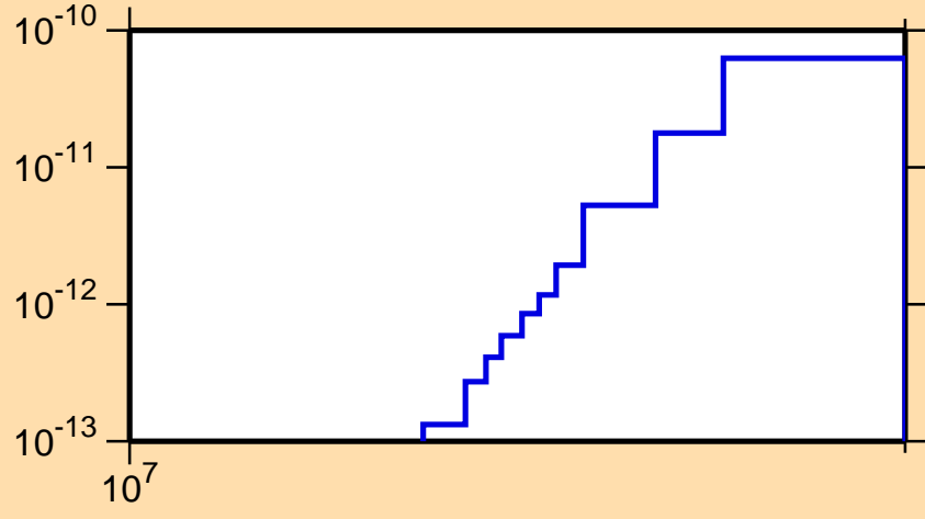
\sigma vs. E for ^{260}\text{Md}(\text{mt } 45)
