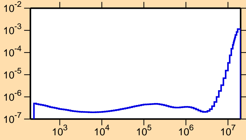
\sigma vs. E for ^{260}\text{Md}(n,\alpha)
