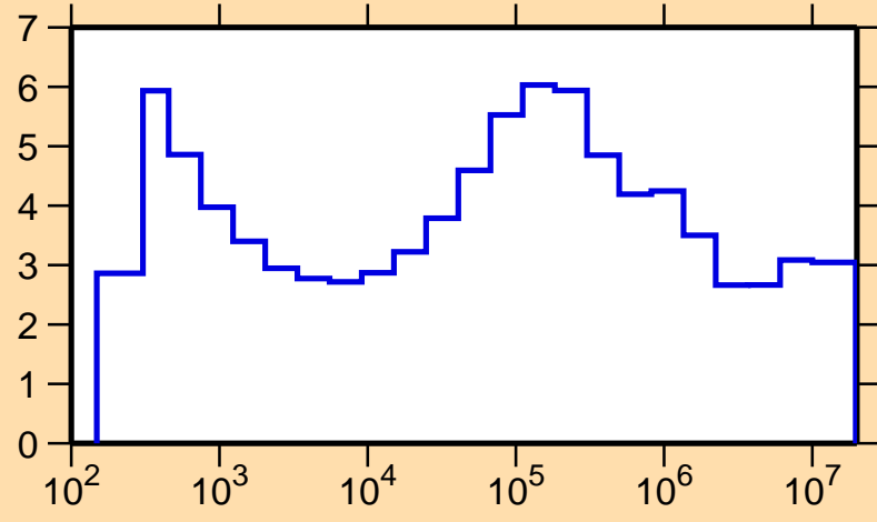
\sigma vs. E for ^{260}\text{Md}(n,\text{nonel.})
