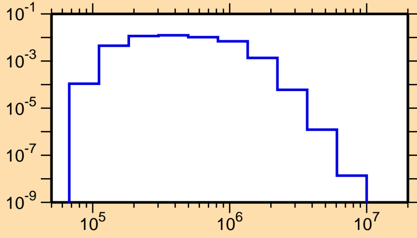
\sigma vs. E for ^{260}\text{Md}(n,n_1)
