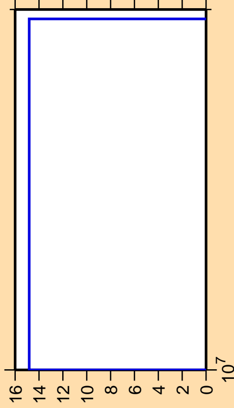
\Delta\sigma/\sigma vs. E for ^{260}\text{Md} (mt 45)
