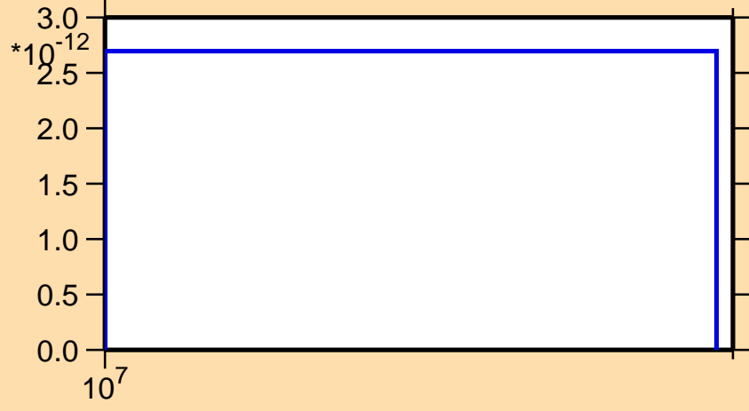
\sigma vs. E for ^{260}\text{Md} (mt 45)
