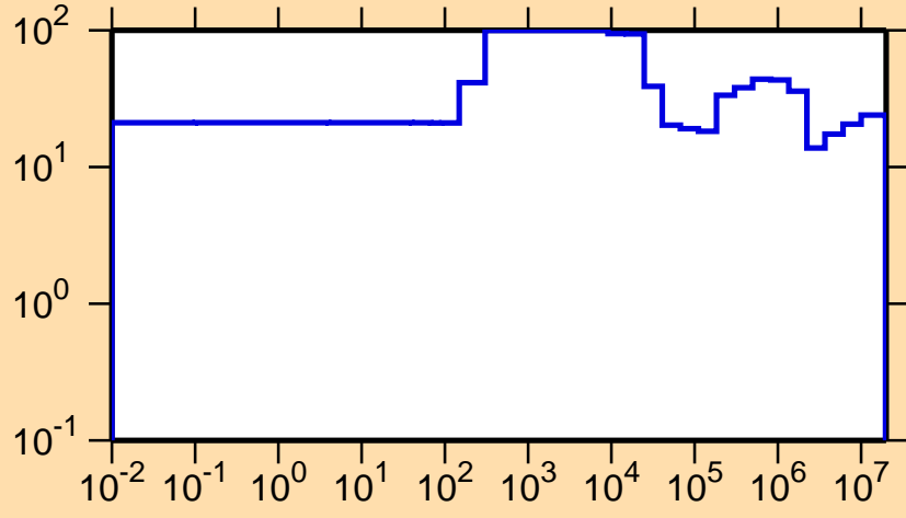
\Delta\sigma/\sigma vs. E for ^{260}\text{Md}(n,el.)
