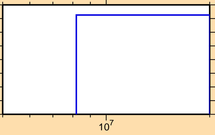
\sigma vs. E for ^{260}\text{Md}(n,3n\alpha)
