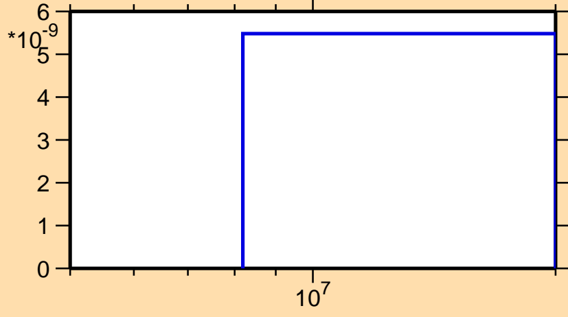
\sigma vs. E for ^{260}\text{Md}(n,2np)
