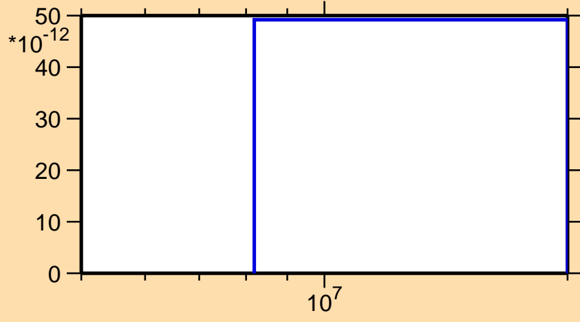
\sigma vs. E for ^{260}\text{Md}(\text{mt117})
