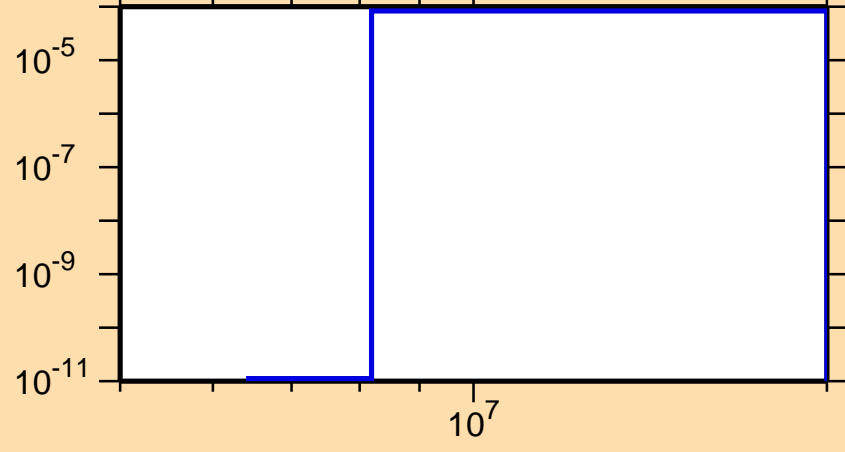
\sigma vs. E for ^{260}\text{Md}(n,t)
