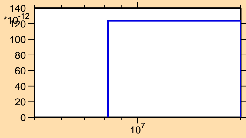
\sigma vs. E for ^{260}\text{Md}(n,p\alpha)
