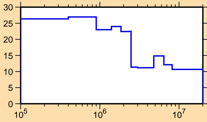
\Delta\sigma/\sigma vs. E for ^{260}\text{Md}(n,\text{tot.})
