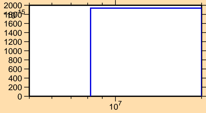
\sigma vs. E for ^{260}\text{Md}(n,\text{He3})
