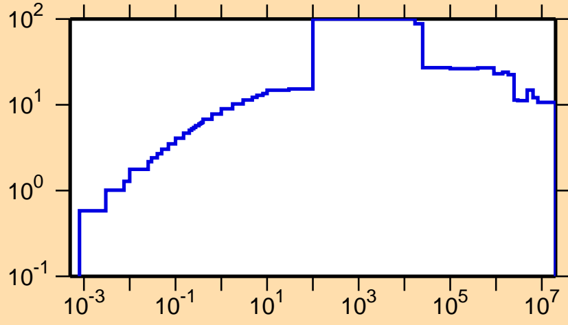
\Delta\sigma/\sigma vs. E for ^{260}\text{Md}(n,\text{tot.})
