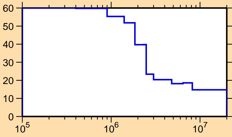
\Delta\sigma/\sigma vs. E for ^{260}\text{Md}(n,\text{nonel.})
