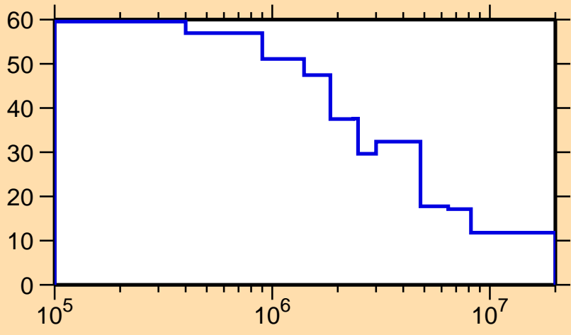
\Delta\sigma/\sigma vs. E for ^{260}\text{Md}(n,f)
