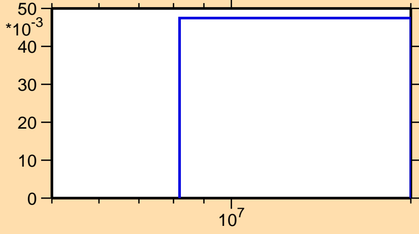
\sigma vs. E for ^{260}\text{Md}(n,3n)
