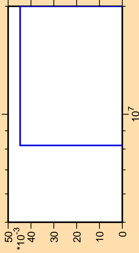
\Delta\sigma/\sigma vs. E for ^{260}\text{Md}(\text{mt } 11)
