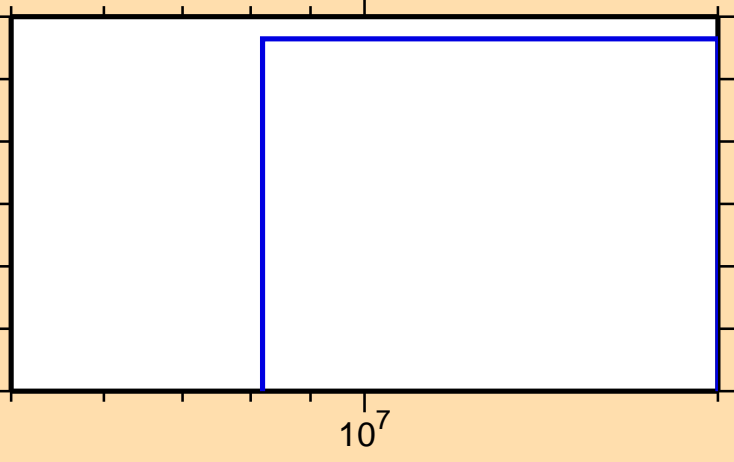
\sigma vs. E for ^{260}\text{Md}(n,nd)
