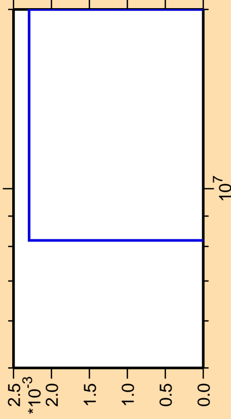
\Delta\sigma/\sigma vs. E for ^{260}\text{Md} (mt 42)
