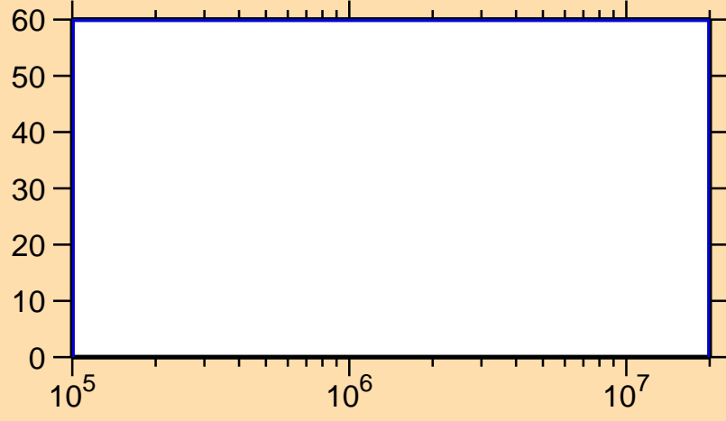
\Delta\sigma/\sigma vs. E for ^{260}\text{Md}(n,n_1)
