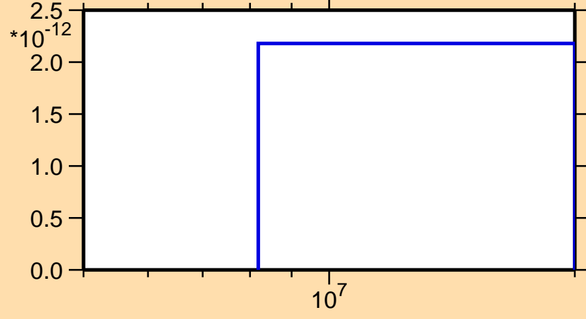
\sigma vs. E for ^{260}\text{Md}(\text{mt } 45)
