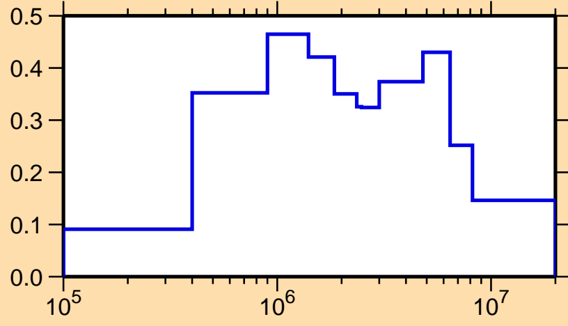
\sigma vs. E for ^{260}\text{Md}(n,\text{inel.})
