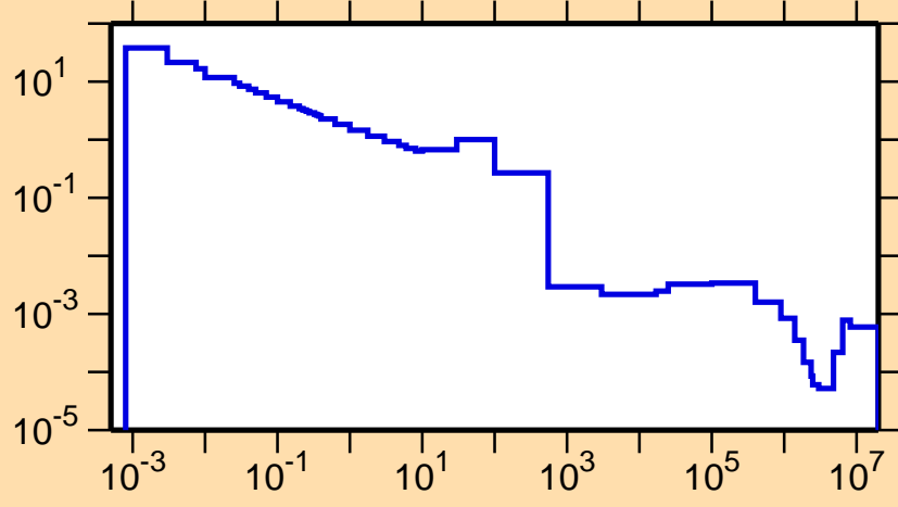
\sigma vs. E for ^{260}\text{Md}(n,\gamma)
