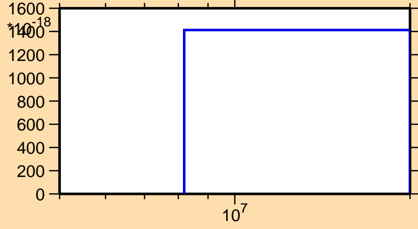
\sigma vs. E for ^{260}\text{Md} (mt 42)
