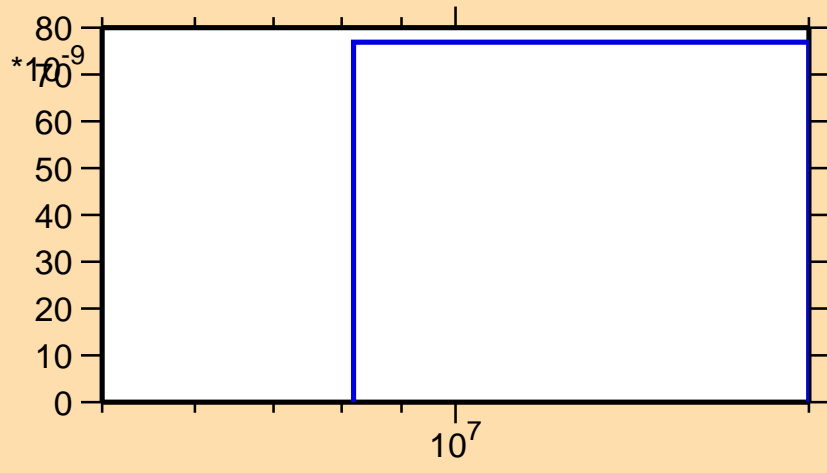
\sigma vs. E for ^{260}\text{Md}(n,nt)
