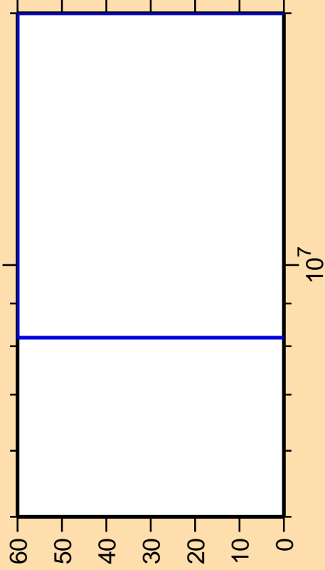
\Delta\sigma/\sigma vs. E for ^{260}\text{Md}(n,p\alpha)
