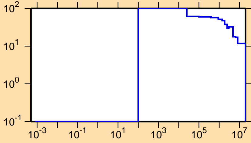
\Delta\sigma/\sigma vs. E for ^{260}\text{Md}(n,f)
