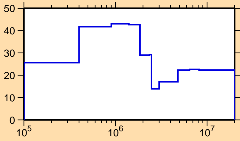
\Delta\sigma/\sigma vs. E for ^{260}\text{Md}(n,\text{el.})
