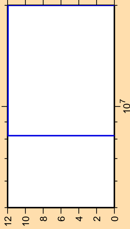
\Delta\sigma/\sigma vs. E for ^{260}\text{Md}(\text{mt } 45)
