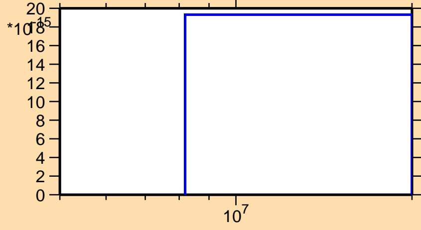
\sigma vs. E for ^{260}\text{Md}(\text{mt } 11)
