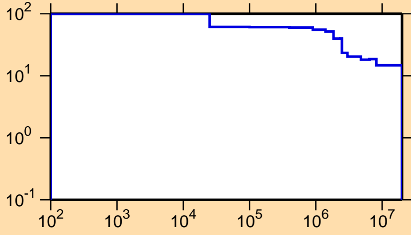
\Delta\sigma/\sigma vs. E for ^{260}\text{Md}(n,\text{nonel.})
