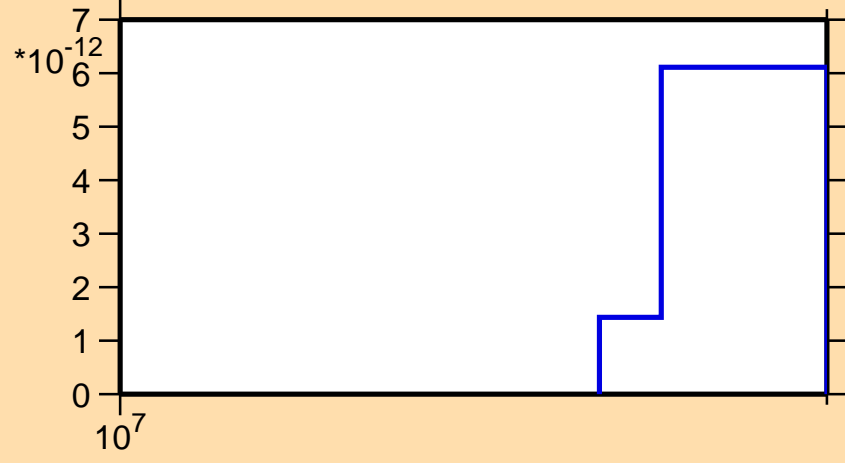
\sigma vs. E for ^{261}\text{Md} (mt 45)
