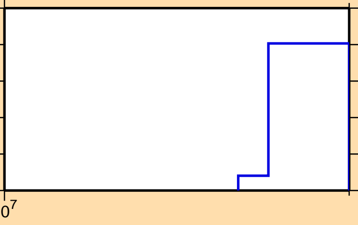
\sigma vs. E for ^{261}\text{Md} (mt 11)
