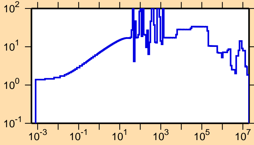
\Delta\sigma/\sigma vs. E for ^{261}\text{Md}(n,tot.)
