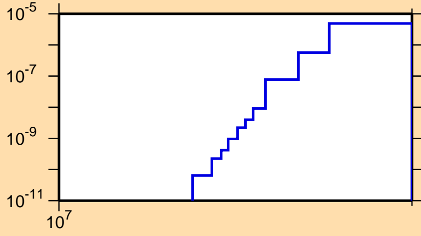
\sigma vs. E for ^{261}\text{Md}(n,nt)
