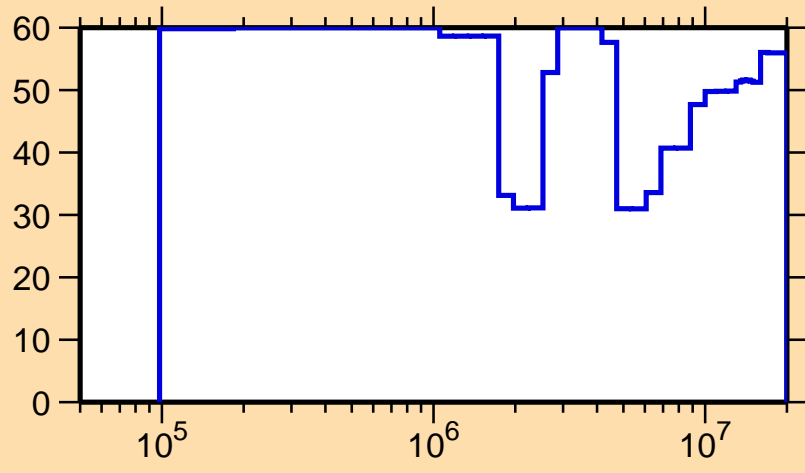
\Delta\sigma/\sigma vs. E for ^{261}\text{Md}(n,n_1)
