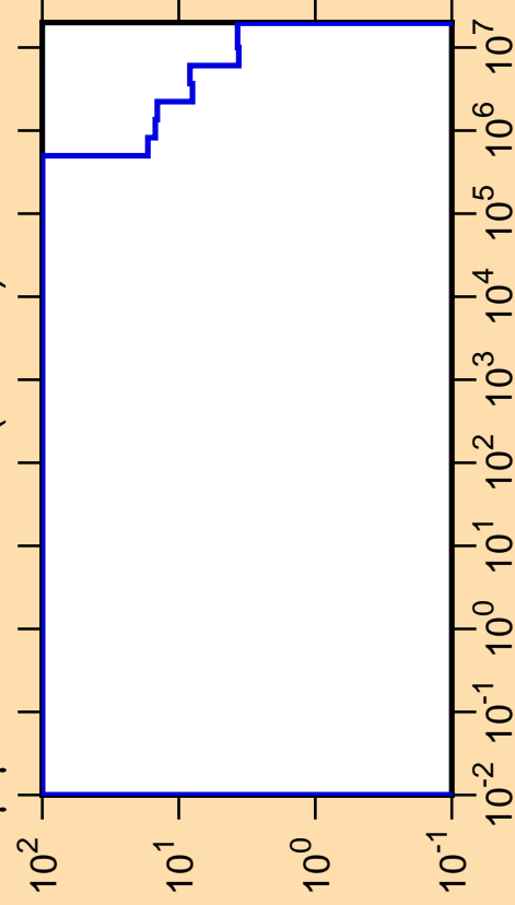
\Delta\mu/\mu vs. E for ^{261}\text{Md}(\text{mt251})
