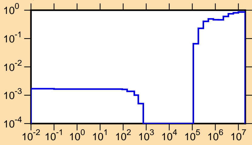
\mu vs. E for ^{261}\text{Md}(\text{mt251})
