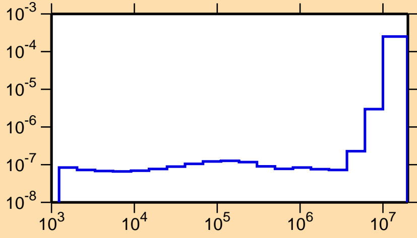
\sigma vs. E for ^{261}\text{Md}(n,\alpha)
