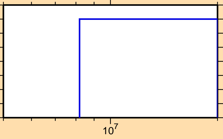
\sigma vs. E for ^{261}\text{Md}(n,3n)
