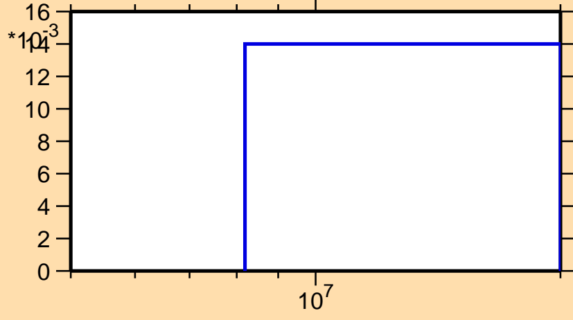
\sigma vs. E for ^{261}\text{Md}(n,3n)
