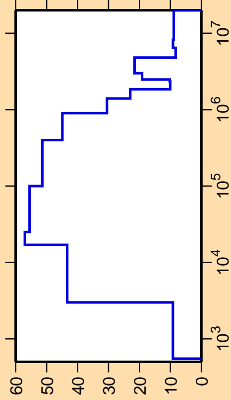
\Delta\sigma/\sigma vs. E for ^{261}\text{Md}(n,\text{nonel.})
