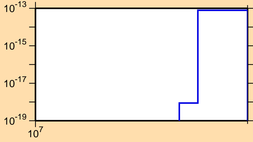
\sigma vs. E for ^{262}\text{Md} (mt 11)
