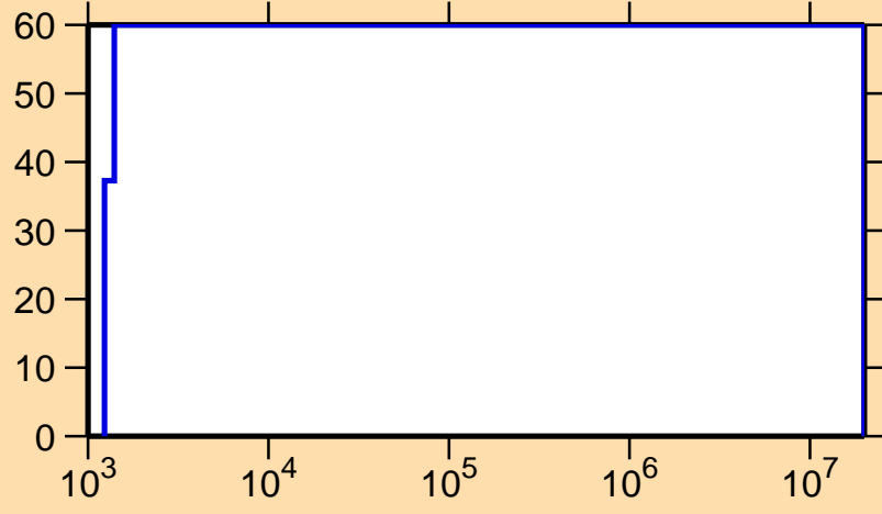
\Delta\sigma/\sigma vs. E for ^{262}\text{Md}(n,\gamma)
