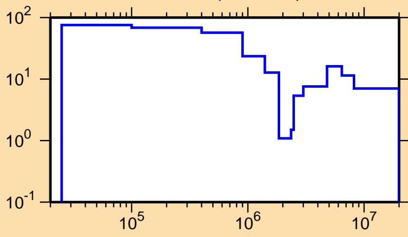
\Delta\sigma/\sigma vs. E for ^{262}\text{Md}(n,n\text{onel.})
