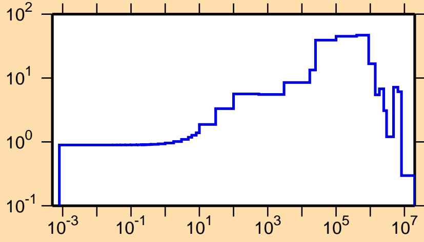
\Delta\sigma/\sigma vs. E for ^{262}\text{Md}(n,tot.)
