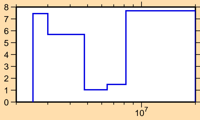
\Delta\sigma/\sigma vs. E for ^{262}\text{Md}(n,\text{el.})
