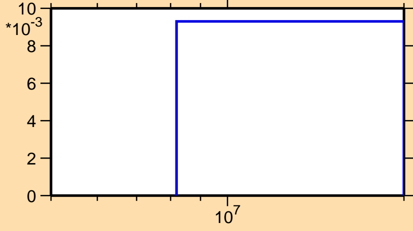
\sigma vs. E for ^{262}\text{Md}(n,3n)
