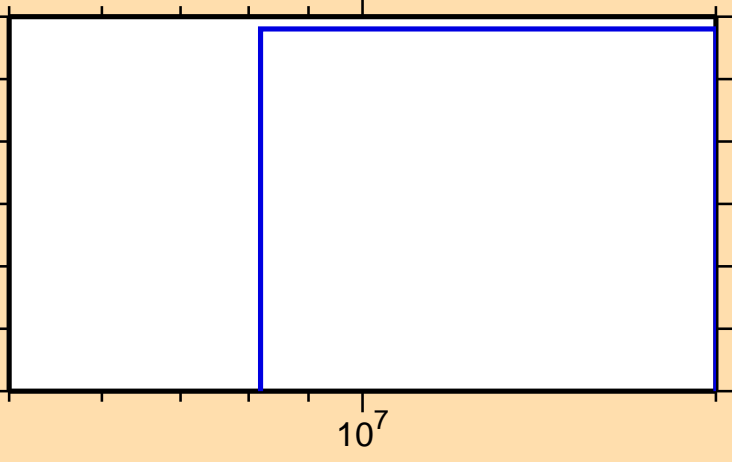
\sigma vs. E for ^{22}\text{Mg}(\text{mt117})
