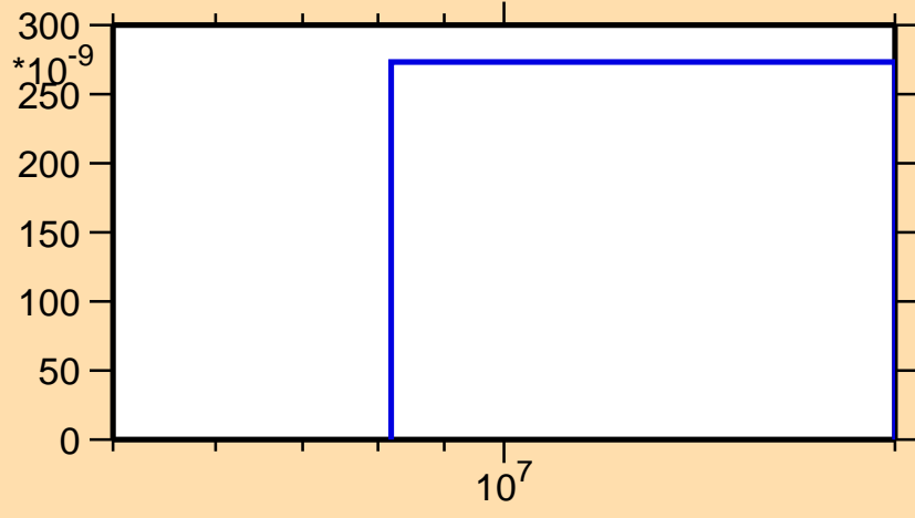
\sigma vs. E for ^{22}\text{Mg}(\text{mt } 45)
