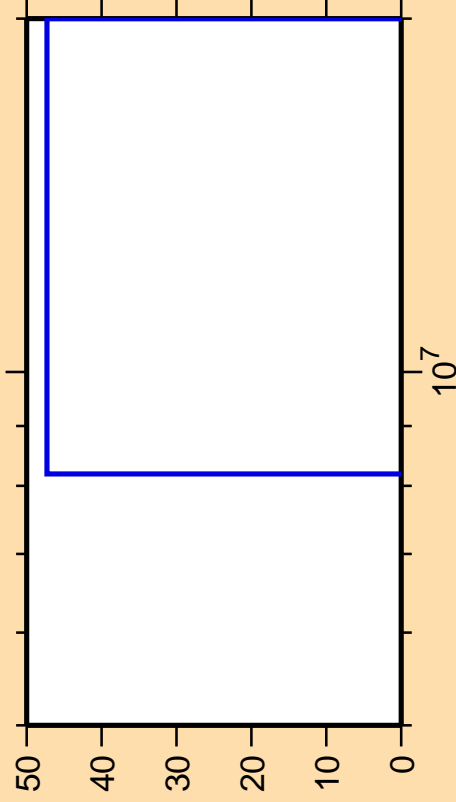
\Delta\sigma/\sigma vs. E for ^{23}\text{Mg}(n,nd)
