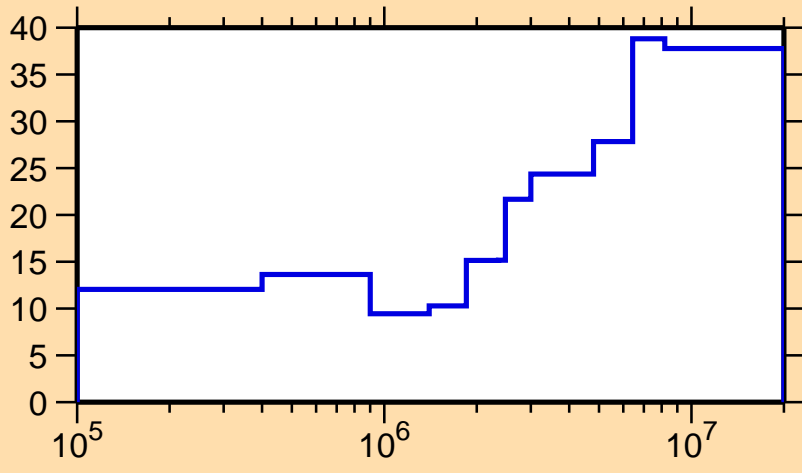
\Delta\sigma/\sigma vs. E for ^{23}\text{Mg}(n,p)
