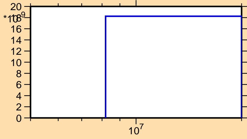
\sigma vs. E for ^{23}\text{Mg}(n,nd)
