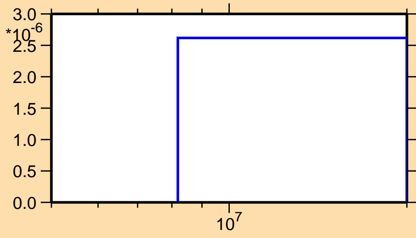
\sigma vs. E for ^{23}\text{Mg}(\text{mt } 34)
