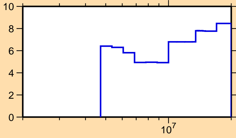
\Delta\sigma/\sigma vs. E for ^{24}\text{Mg}(n,el.)
