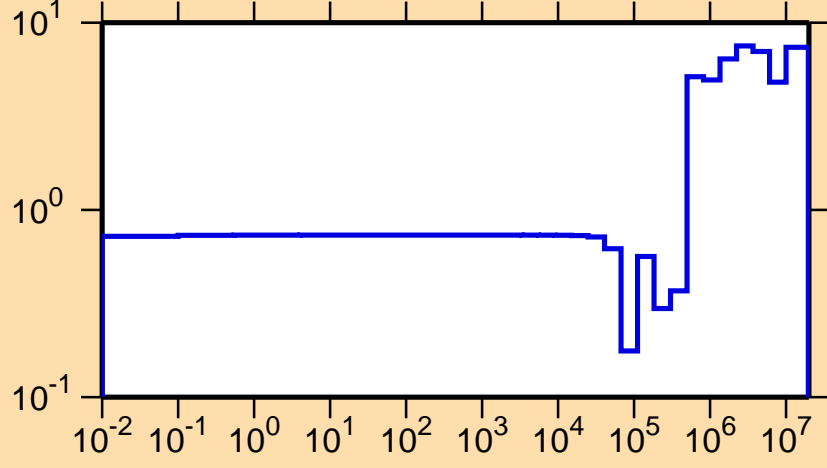
\Delta\sigma/\sigma vs. E for ^{24}\text{Mg}(n,\text{el.})
