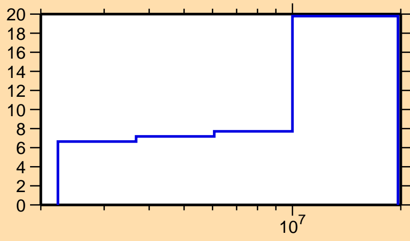
\Delta\sigma/\sigma vs. E for ^{24}\text{Mg}(n,n_1)
