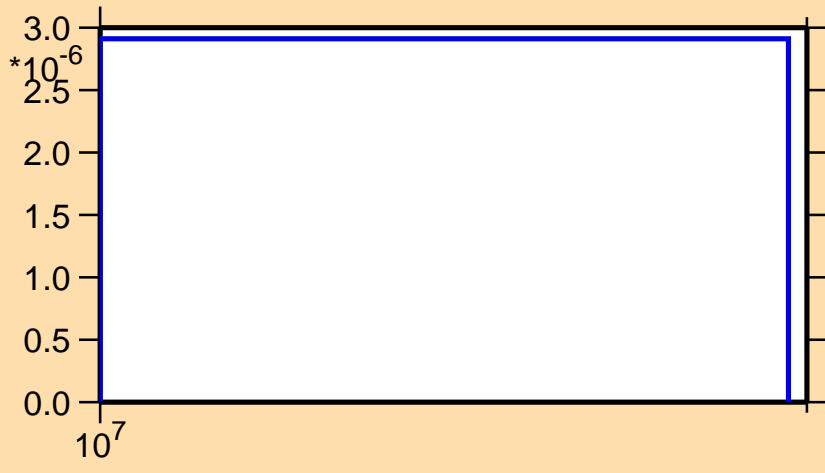
\sigma vs. E for ^{24}\text{Mg}(n,\text{He}3)
