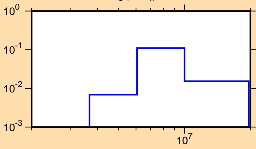
\sigma vs. E for ^{24}\text{Mg}(n,n_4)
