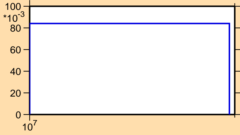
\sigma vs. E for ^{24}\text{Mg}(n,np)
