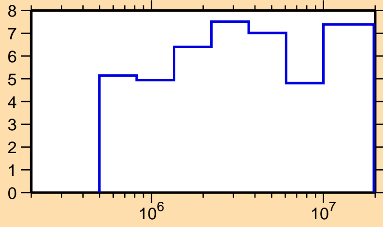
\Delta\sigma/\sigma vs. E for ^{24}\text{Mg}(n,\text{el.})
