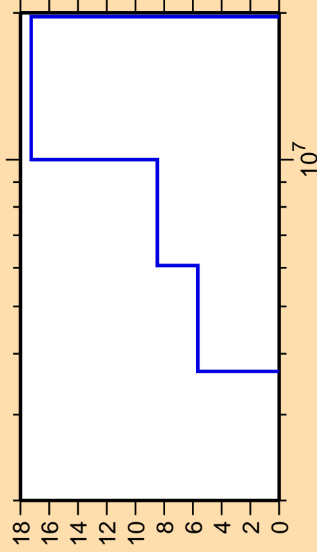
\Delta\sigma/\sigma vs. E for ^{24}\text{Mg}(n,n_3)
