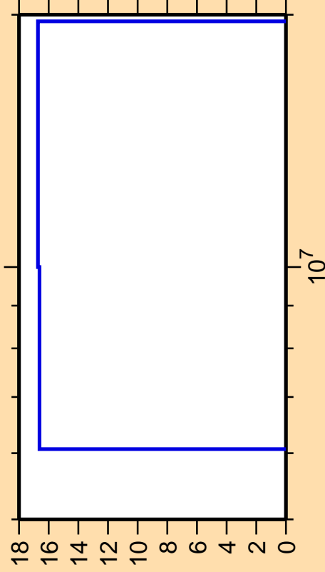
\Delta\sigma/\sigma vs. E for ^{24}\text{Mg}(n,n\alpha)
