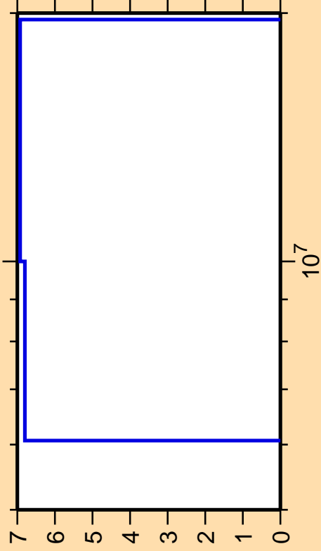
\Delta\sigma/\sigma vs. E for ^{24}\text{Mg}(n,p)
