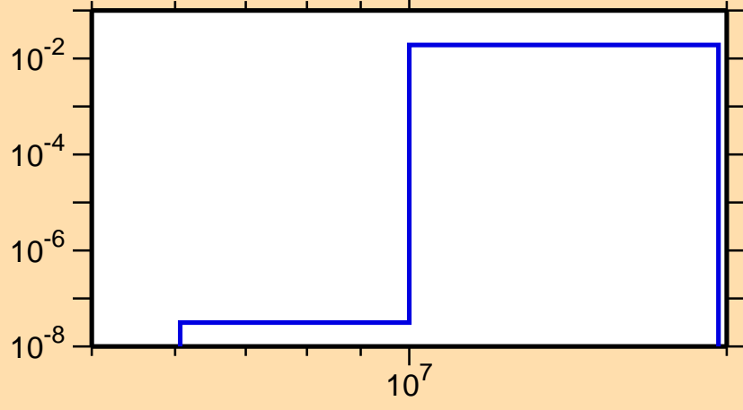
\sigma vs. E for ^{24}\text{Mg}(n,d)
