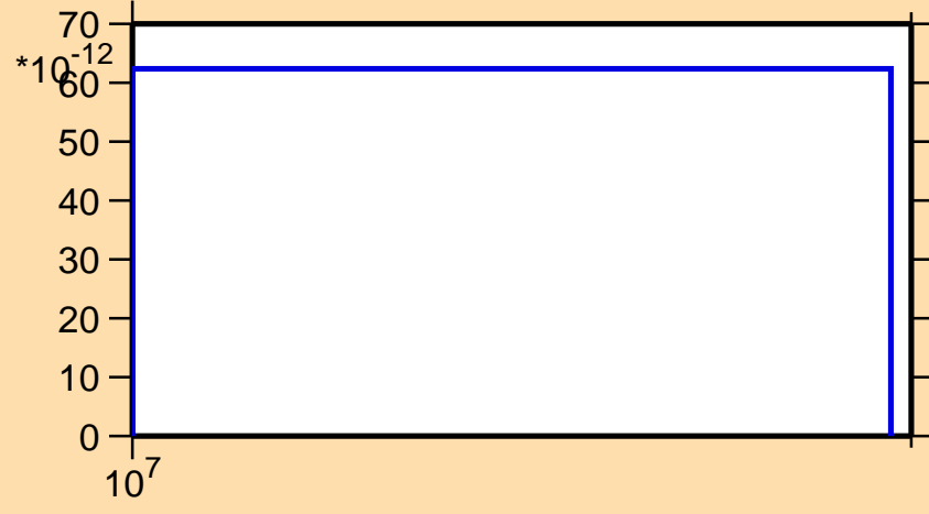
\sigma vs. E for ^{24}\text{Mg}(n,p\alpha)
