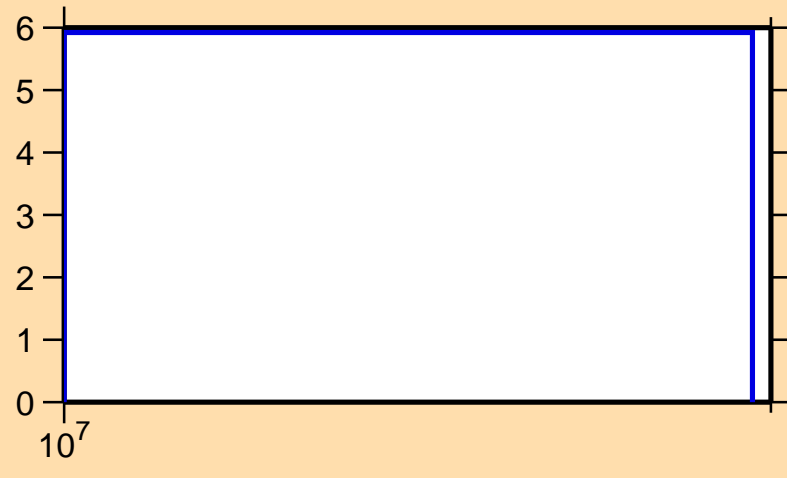
\Delta\sigma/\sigma vs. E for ^{24}\text{Mg}(n,\text{nonel.})
