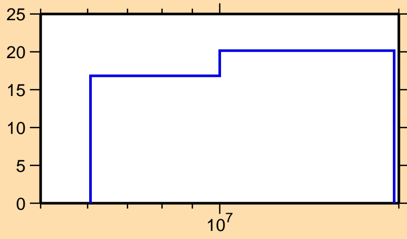
\Delta\sigma/\sigma vs. E for ^{24}\text{Mg}(n,n\text{cont.})
