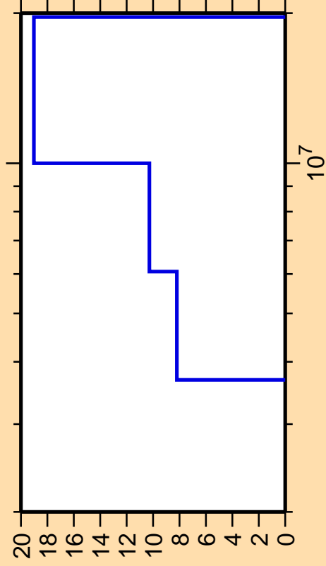
\Delta\sigma/\sigma vs. E for ^{24}\text{Mg}(n,n_2)
