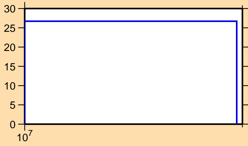
\Delta\sigma/\sigma vs. E for ^{24}\text{Mg}(n,2n)
