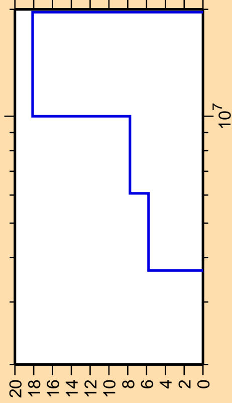
\Delta\sigma/\sigma vs. E for ^{24}\text{Mg}(n,n_4)
