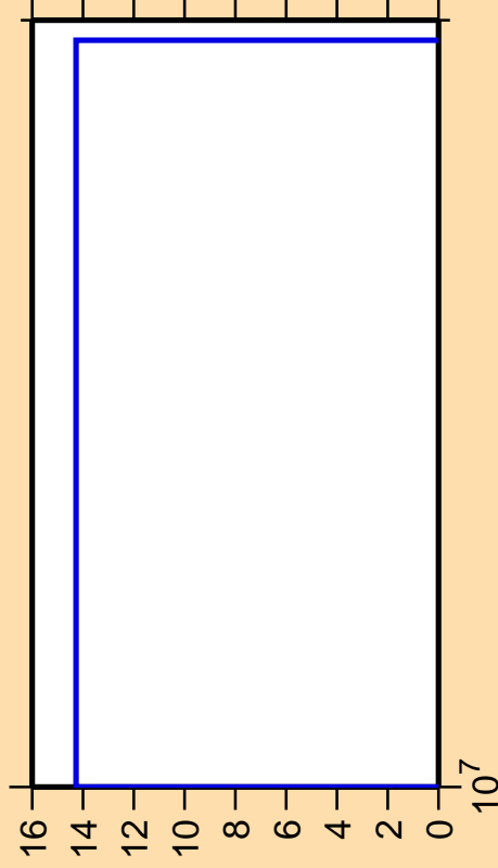
\Delta\sigma/\sigma vs. E for ^{24}\text{Mg}(n,np)
