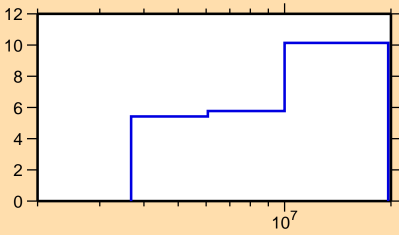
\Delta\sigma/\sigma vs. E for ^{24}\text{Mg}(n,\text{inel.})
