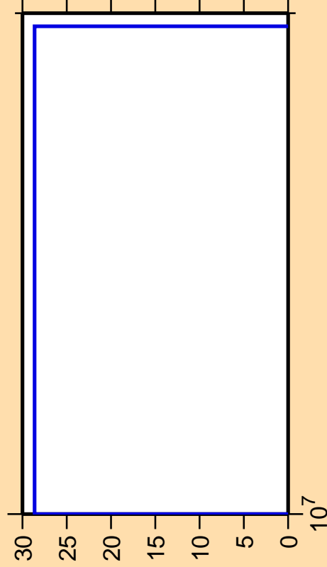
\Delta\sigma/\sigma vs. E for ^{24}\text{Mg}(n,p\alpha)
