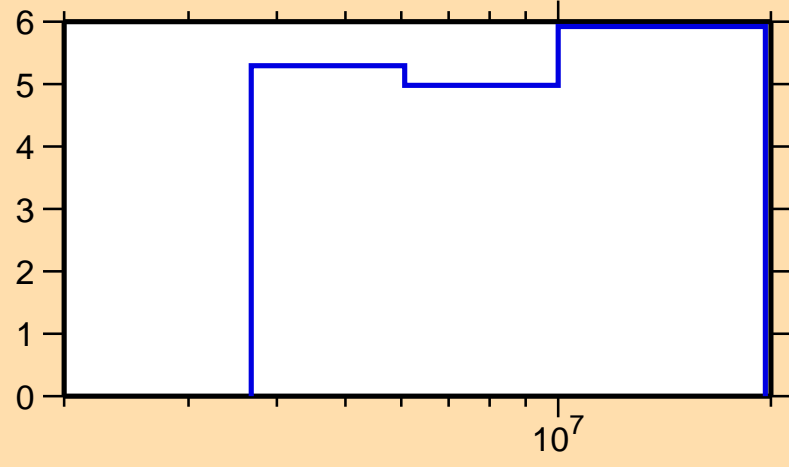
\Delta\sigma/\sigma vs. E for ^{24}\text{Mg}(n,\text{nonel.})
