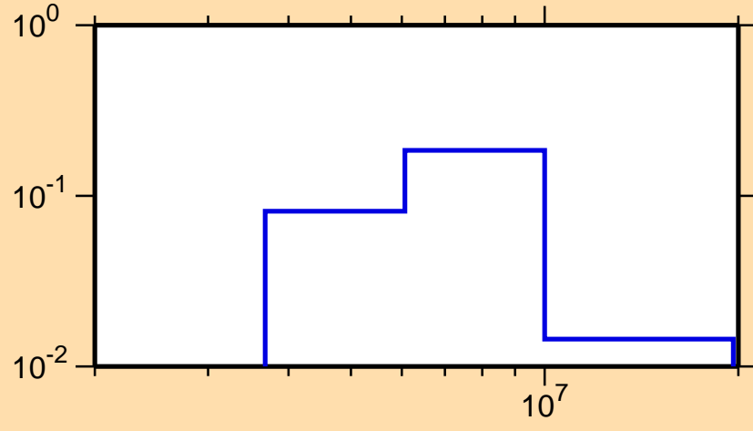
\sigma vs. E for ^{24}\text{Mg}(n,n_3)
