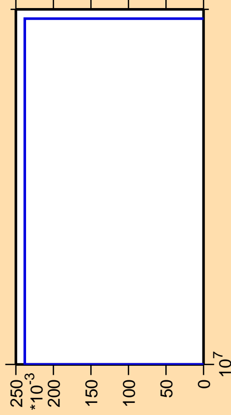
\Delta\sigma/\sigma vs. E for ^{24}\text{Mg}(n,pd)
