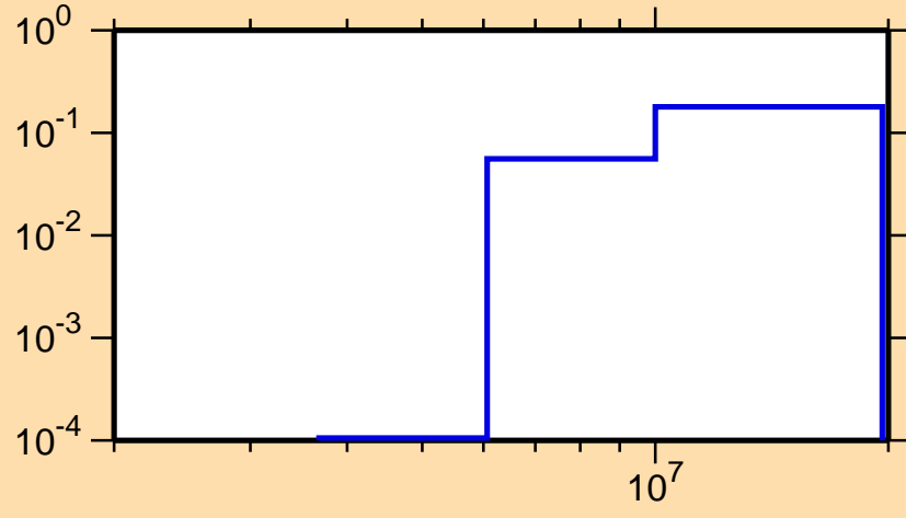
\sigma vs. E for ^{24}\text{Mg}(n,p)
