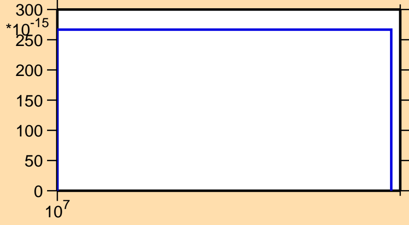
\sigma vs. E for ^{24}\text{Mg}(n,pd)
