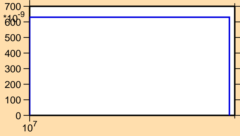
\sigma vs. E for ^{24}\text{Mg}(n,t)
