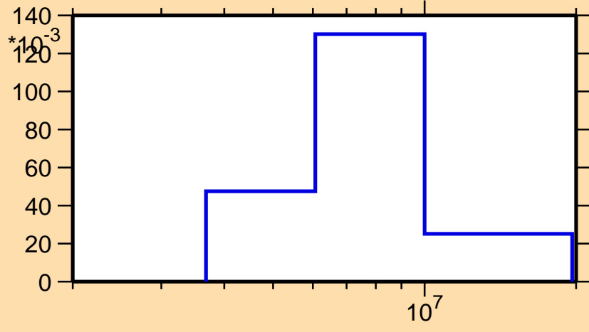
\sigma vs. E for ^{24}\text{Mg}(n,n_2)
