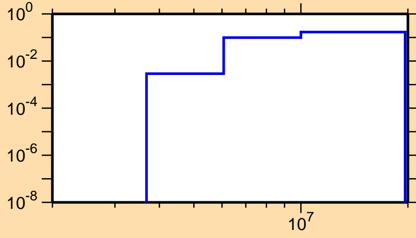
\sigma vs. E for ^{24}\text{Mg}(n,\alpha)
