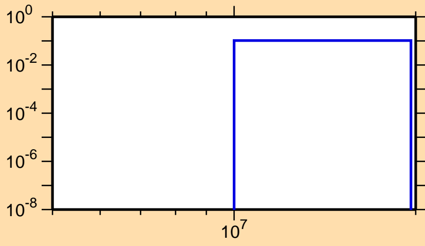
\sigma vs. E for ^{24}\text{Mg}(n,n\alpha)
