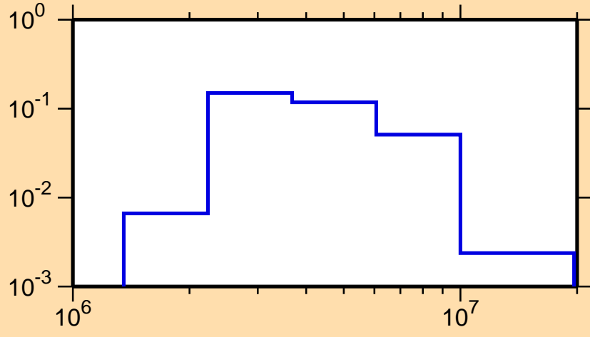
\sigma vs. E for ^{25}\text{Mg}(n,n_4)
