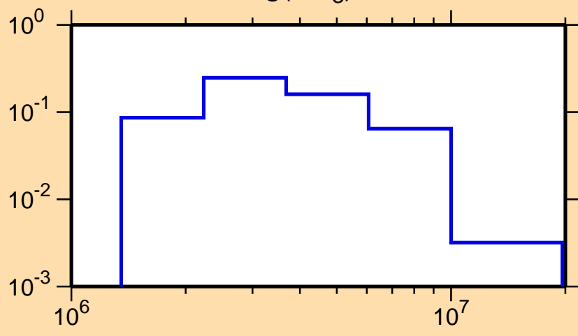
\sigma vs. E for ^{25}\text{Mg}(n,n_3)
