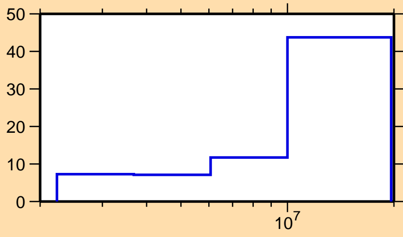
\Delta\sigma/\sigma vs. E for ^{25}\text{Mg}(n,n_1)
