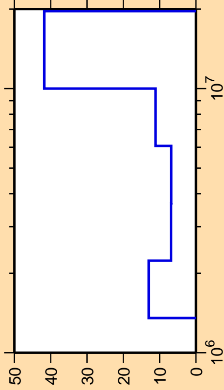
\Delta\sigma/\sigma vs. E for ^{25}\text{Mg}(n,n_4)
