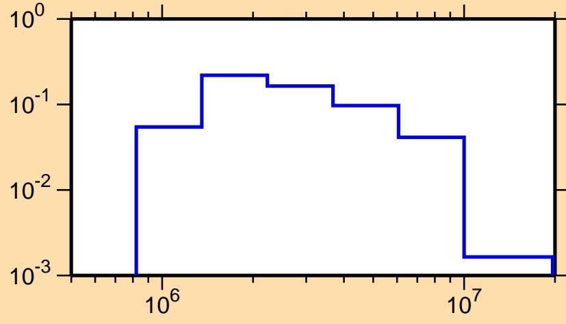
\sigma vs. E for ^{25}\text{Mg}(n,n_2)
