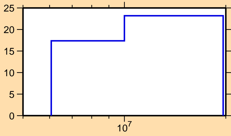
\Delta\sigma/\sigma vs. E for ^{25}\text{Mg}(n,n\text{cont.})
