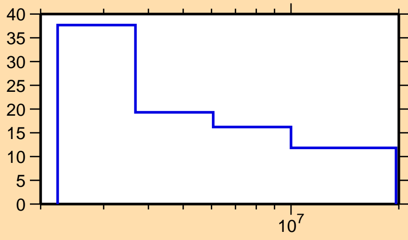
\Delta\sigma/\sigma vs. E for ^{25}\text{Mg}(n,p)
