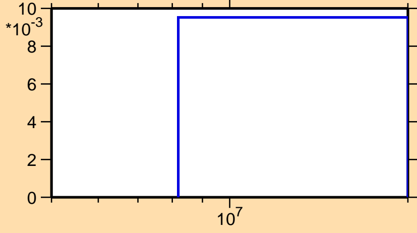
\sigma vs. E for ^{25}\text{Mg}(n,n\alpha)
