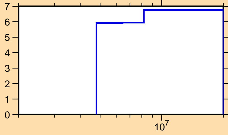
\Delta\sigma/\sigma vs. E for ^{25}\text{Mg}(n,n\text{onl.})
