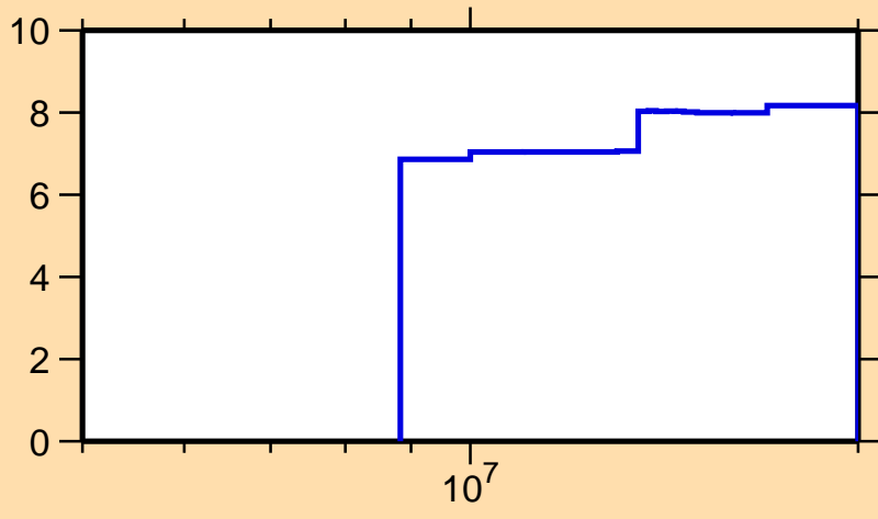
\Delta\sigma/\sigma vs. E for ^{26}\text{Mg}(n,el.)
