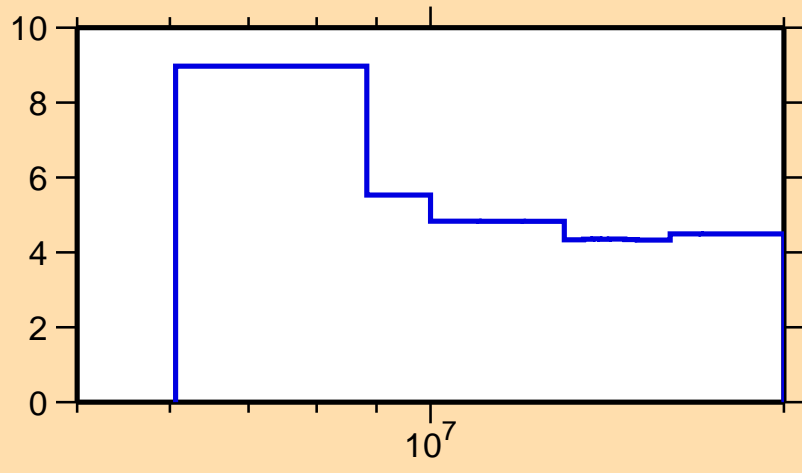
\Delta\sigma/\sigma vs. E for ^{27}\text{Mg}(n,2n)
