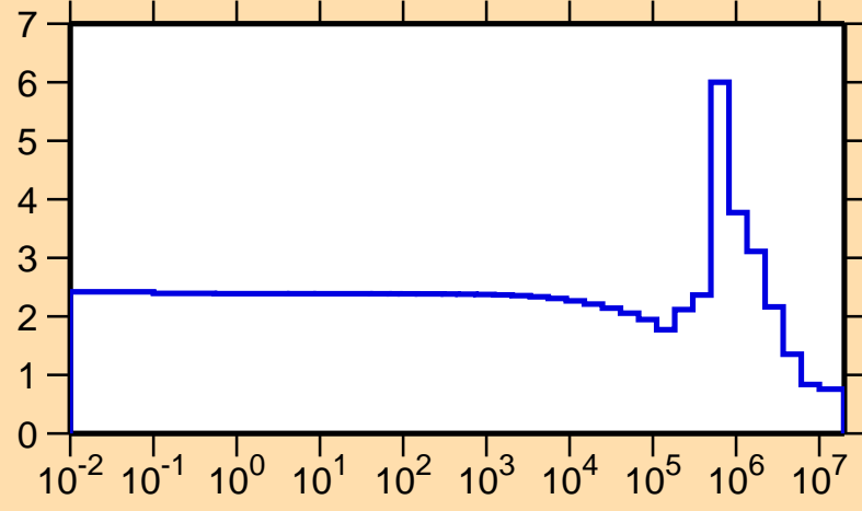
\sigma vs. E for ^{27}\text{Mg}(n,\text{el.})
