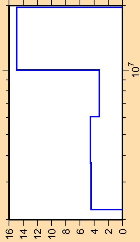
\Delta\sigma/\sigma vs. E for ^{27}\text{Mg}(n,n_4)
