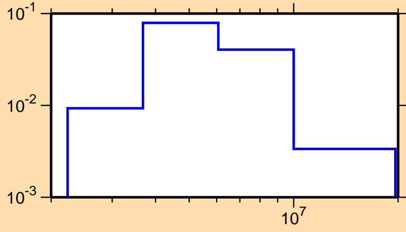
\sigma vs. E for ^{27}\text{Mg}(n,n_4)
