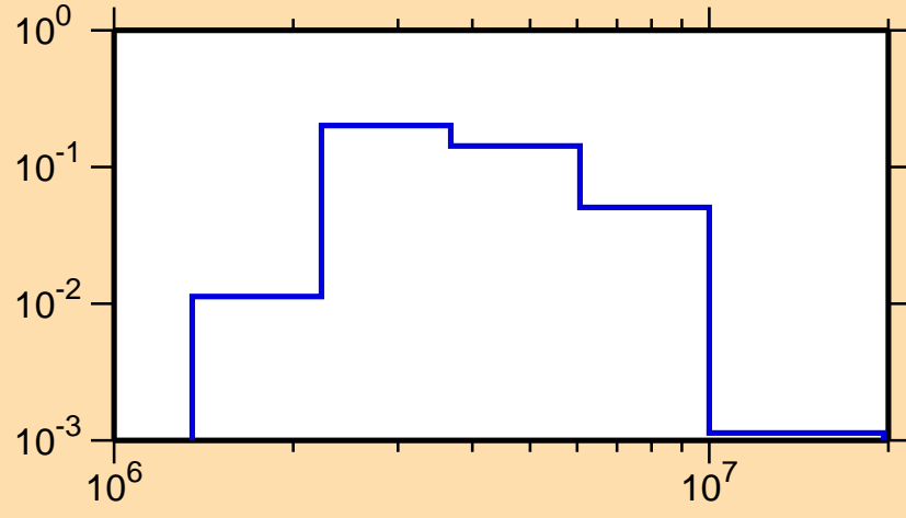
\sigma vs. E for ^{27}\text{Mg}(n,n_3)
