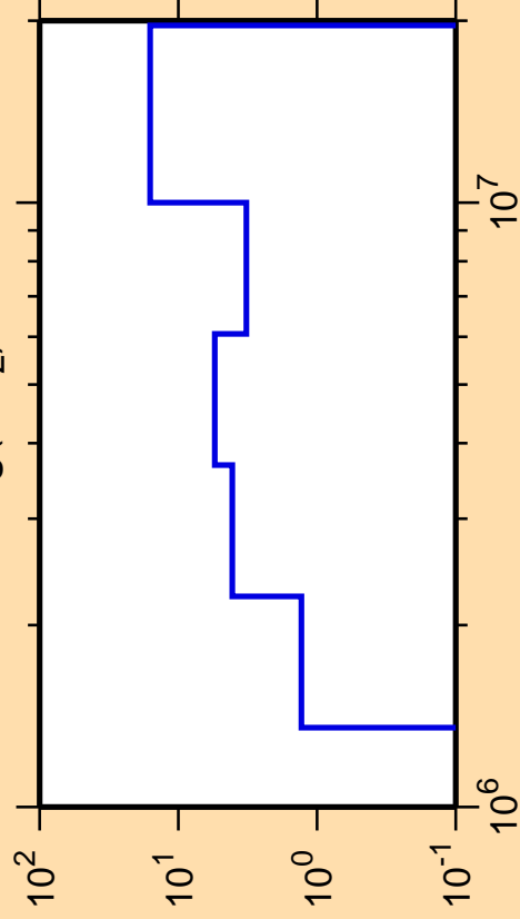
\Delta\sigma/\sigma vs. E for ^{27}\text{Mg}(n,n_2)
