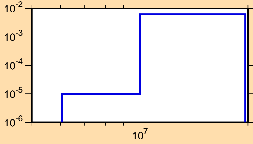
\sigma vs. E for ^{27}\text{Mg}(n,p)
