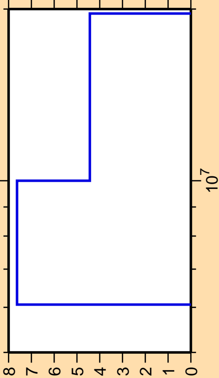
\Delta\sigma/\sigma vs. E for ^{27}\text{Mg}(n,2n)
