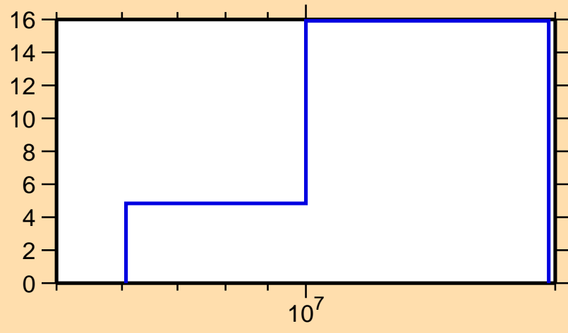
\Delta\sigma/\sigma vs. E for ^{27}\text{Mg}(n,n\text{cont.})
