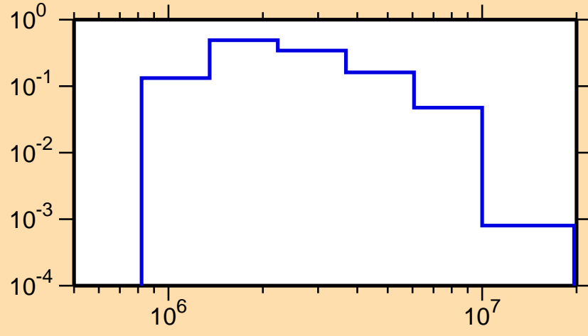
\sigma vs. E for ^{27}\text{Mg}(n,n_1)
