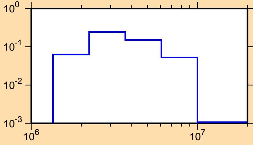
\sigma vs. E for ^{27}\text{Mg}(n,n_2)
