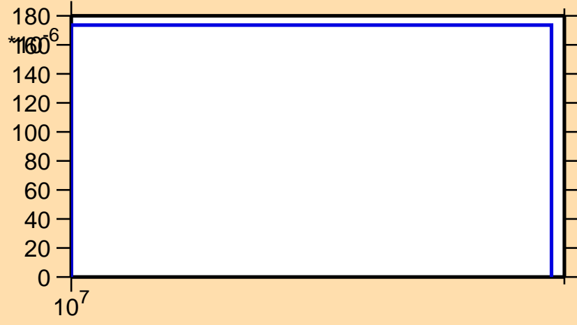
\sigma vs. E for ^{27}\text{Mg}(n,n\alpha)
