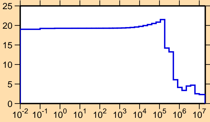
\Delta\sigma/\sigma vs. E for ^{27}\text{Mg}(n,\text{el.})
