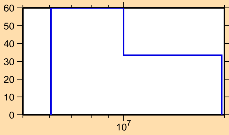
\Delta\sigma/\sigma vs. E for ^{27}\text{Mg}(n,\gamma)
