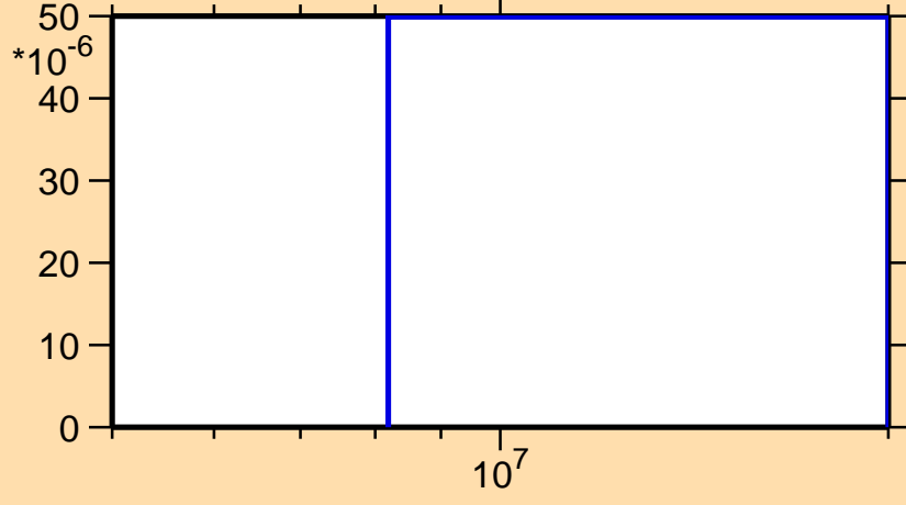
\sigma vs. E for ^{27}\text{Mg}(n,d)
