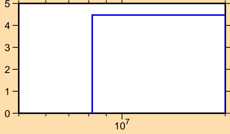
\Delta\sigma/\sigma vs. E for ^{28}\text{Mg}(n,el.)
