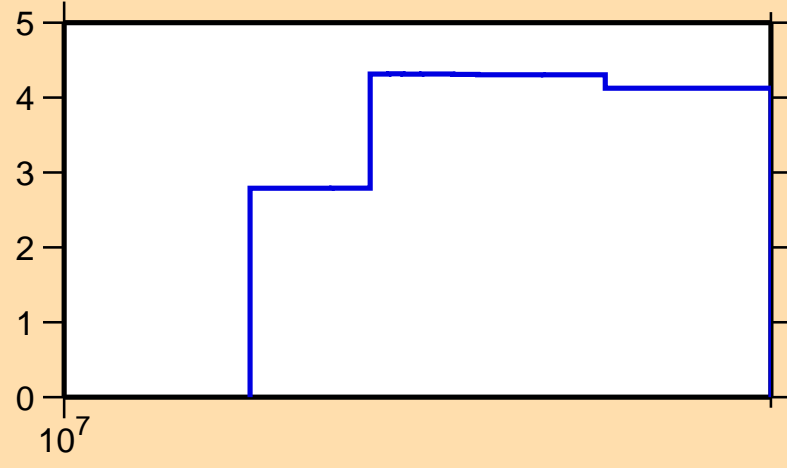
\Delta\sigma/\sigma vs. E for ^{29}\text{Mg}(n,el.)
