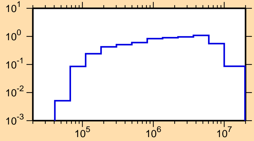
\sigma vs. E for ^{29}\text{Mg}(n,\text{inel.})
