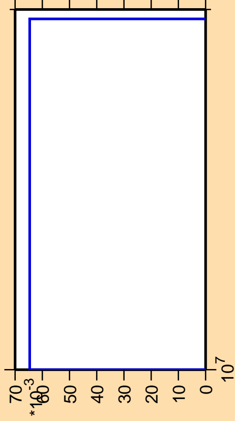
\Delta\sigma/\sigma vs. E for ^{29}\text{Mg}(n,nt)
