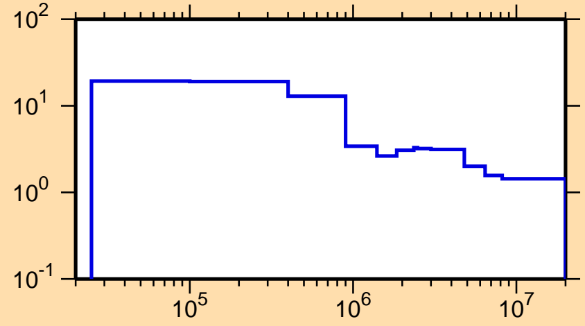
\Delta\sigma/\sigma vs. E for ^{29}\text{Mg}(n,\text{nonel.})
