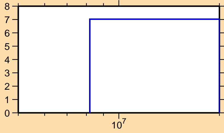
\Delta\sigma/\sigma vs. E for ^{29}\text{Mg}(n,\text{inel.})
