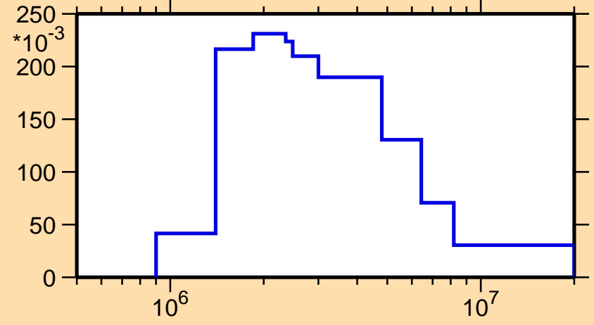
\sigma vs. E for ^{29}\text{Mg}(n,n_3)
