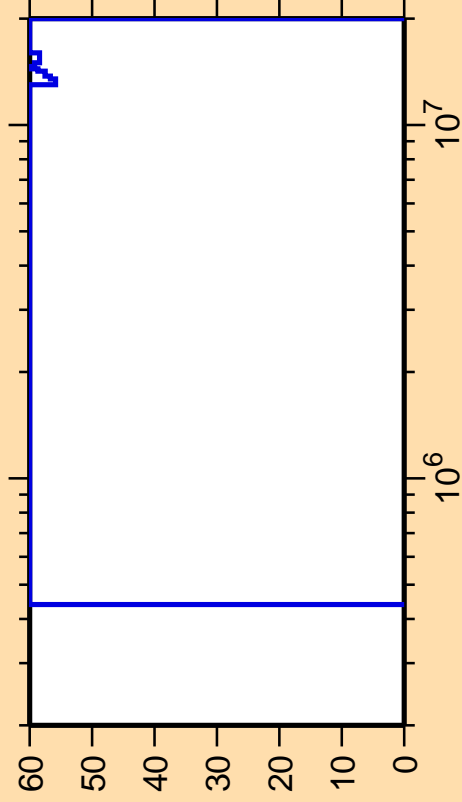
\Delta\sigma/\sigma vs. E for ^{50}\text{Mn}(n,n_2)
