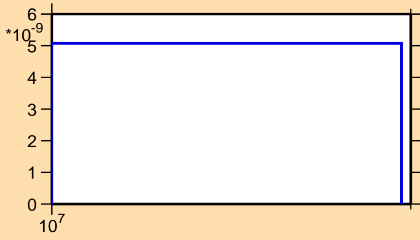
\sigma vs. E for ^{50}\text{Mn}(n,\text{pt})
