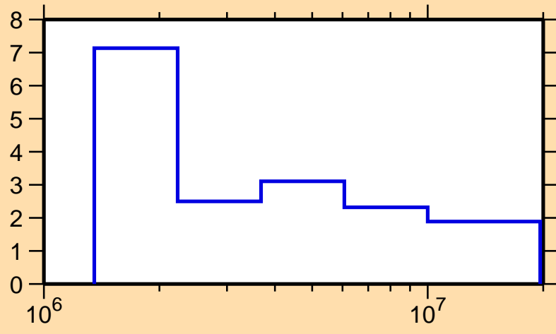
\Delta\sigma/\sigma vs. E for ^{50}\text{Mn}(n,\text{nonel.})
