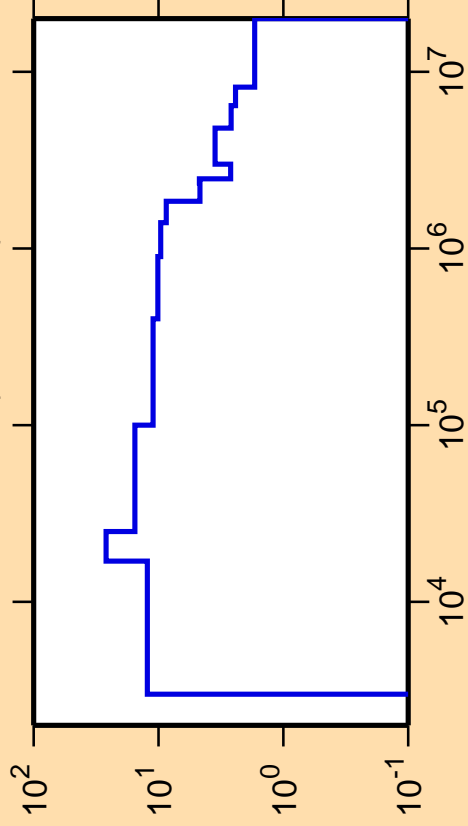
\Delta\sigma/\sigma vs. E for ^{50}\text{Mn}(n,\text{nonel.})
