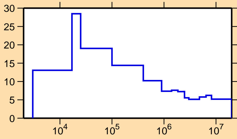
\Delta\sigma/\sigma vs. E for ^{50}\text{Mn}(n,\text{tot.})
