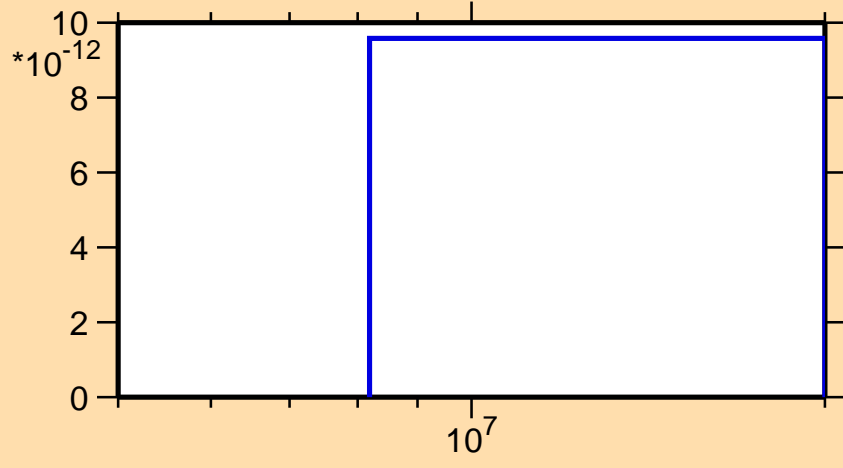
\sigma vs. E for ^{50}\text{Mn} (mt 34)
