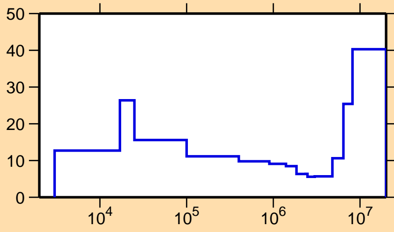
\Delta\sigma/\sigma vs. E for ^{50}\text{Mn}(n,p)
