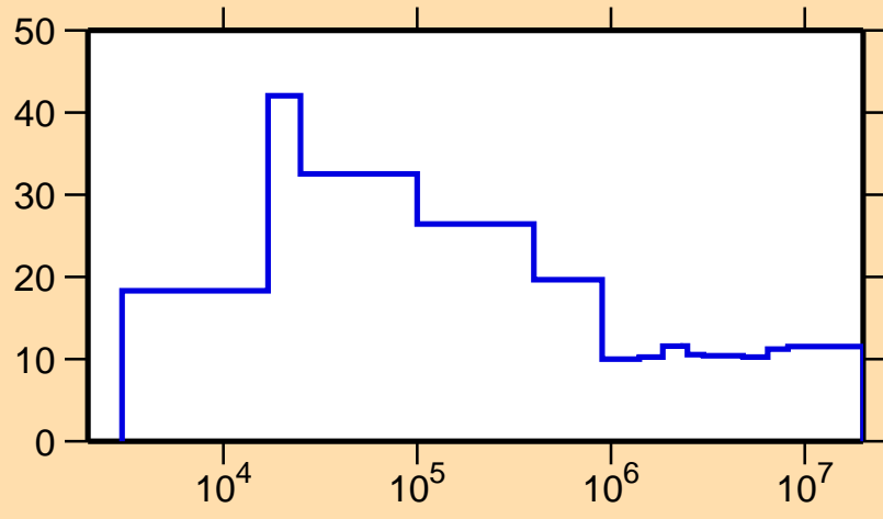
\Delta\sigma/\sigma vs. E for ^{50}\text{Mn}(n,el.)
