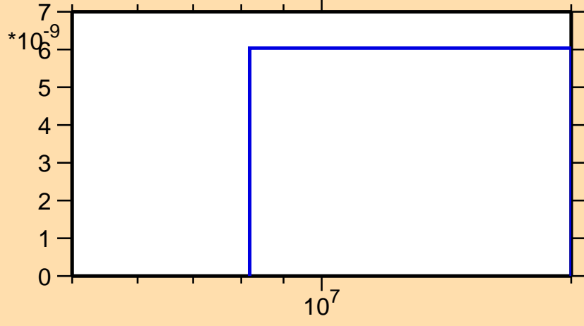
\sigma vs. E for ^{50}\text{Mn}(n,pt)
