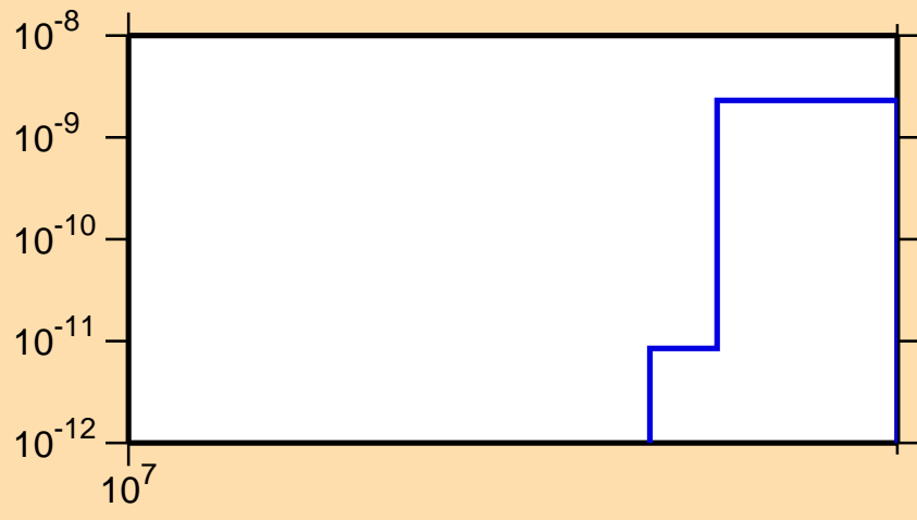
\sigma vs. E for ^{51}\text{Mn}(\text{mt117})
