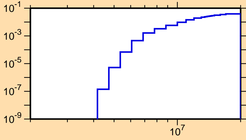
\sigma vs. E for ^{51}\text{Mn}(n,d)
