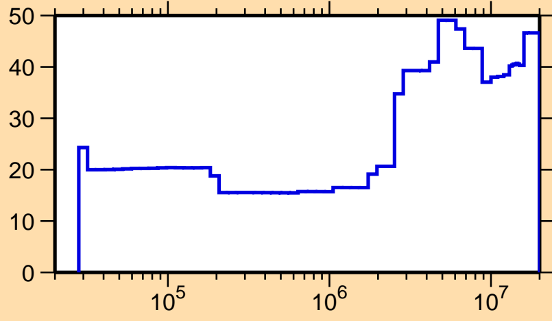
\Delta\sigma/\sigma vs. E for ^{51}\text{Mn}(n,p)
