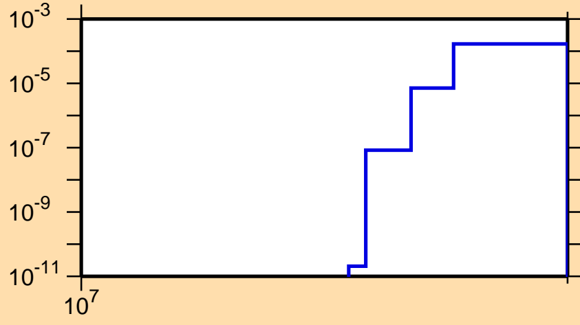
\sigma vs. E for ^{51}\text{Mn}(n,pd)
