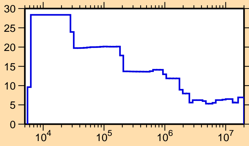
\Delta\sigma/\sigma vs. E for ^{51}\text{Mn}(n,\text{nonel.})
