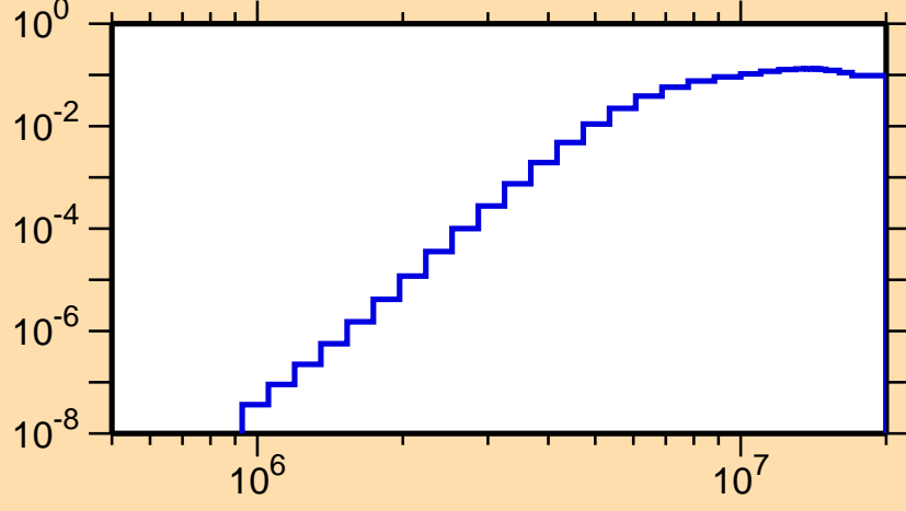
\sigma vs. E for ^{51}\text{Mn}(n,\alpha)
