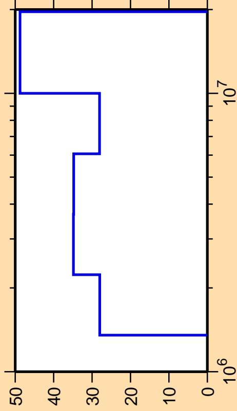
\Delta\sigma/\sigma vs. E for ^{51}\text{Mn}(n,n_3)
