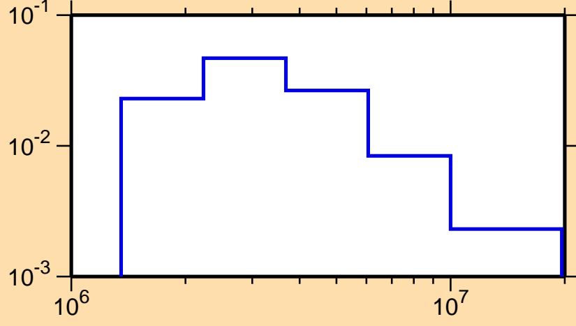
\sigma vs. E for ^{51}\text{Mn}(n,n_3)
