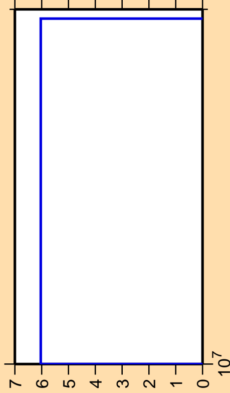
\Delta\sigma/\sigma vs. E for ^{51}\text{Mn} (mt 45)
