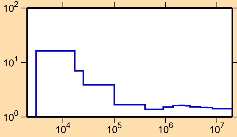
\sigma vs. E for ^{51}\text{Mn}(n,\text{nonel.})
