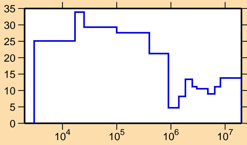
\Delta\sigma/\sigma vs. E for ^{51}\text{Mn}(n,el.)
