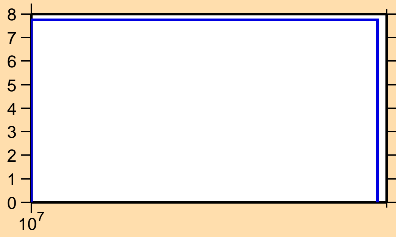
\Delta\sigma/\sigma vs. E for ^{52}\text{Mn}(n,\text{tot.})
