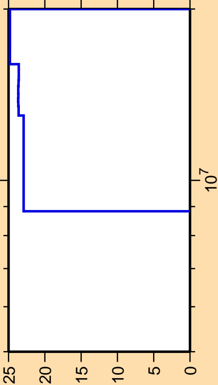
\Delta\sigma/\sigma vs. E for ^{54}\text{Mn}(n,2n)
