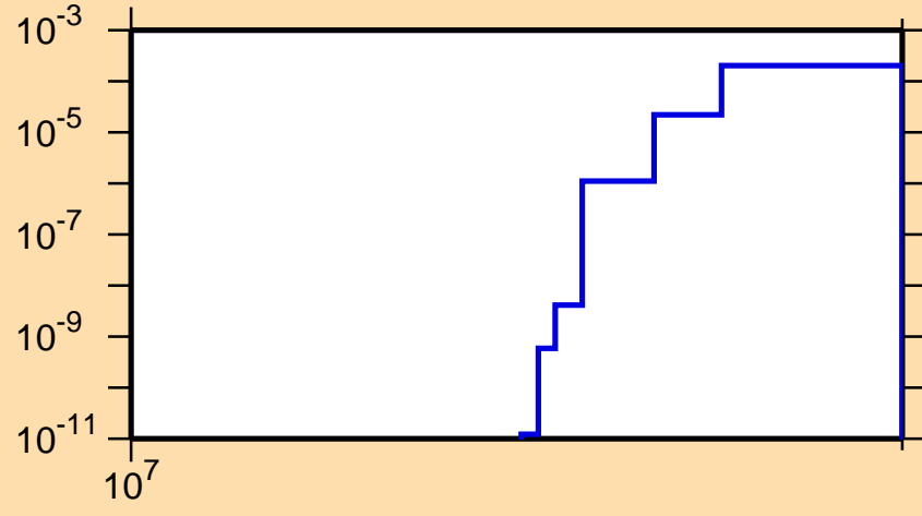
\sigma vs. E for ^{54}\text{Mn}(n,nd)
