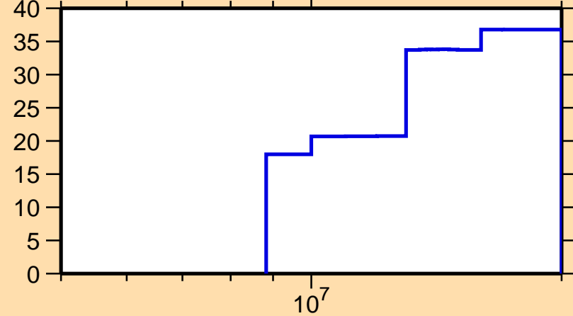
\Delta\sigma/\sigma vs. E for ^{54}\text{Mn}(n,\text{inel.})
