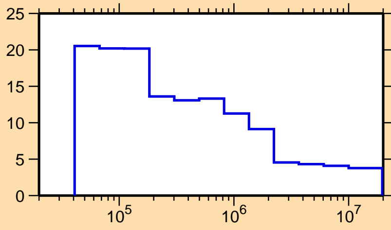
\Delta\sigma/\sigma vs. E for ^{54}\text{Mn}(n,\text{nonel.})
