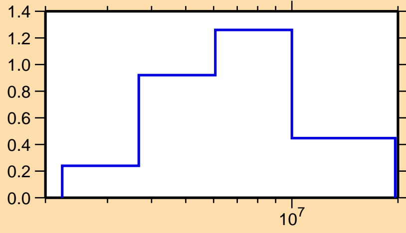
\sigma vs. E for ^{54}\text{Mn}(n,n\text{cont.})
