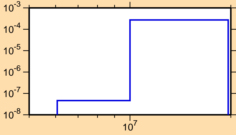
\sigma vs. E for ^{54}\text{Mn}(n,t)
