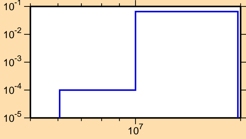
\sigma vs. E for ^{54}\text{Mn}(n,np)
