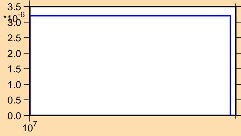
\sigma vs. E for ^{54}\text{Mn}(n,\text{nd})
