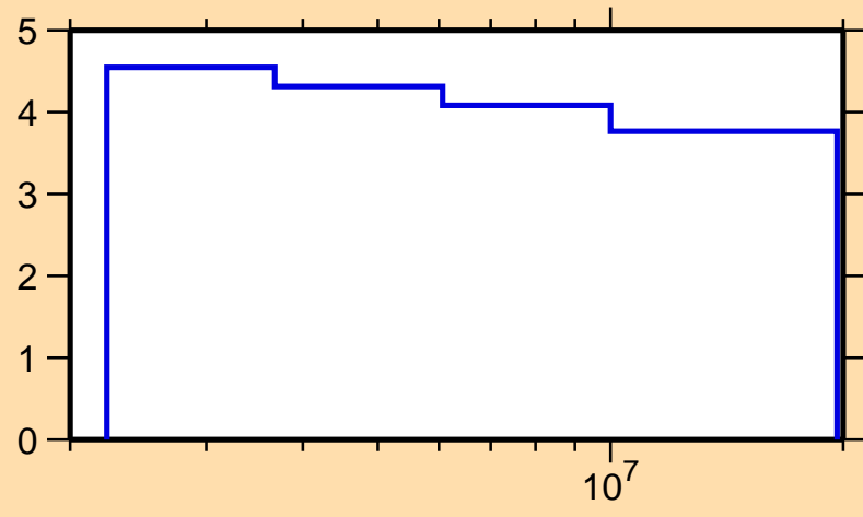
\Delta\sigma/\sigma vs. E for ^{54}\text{Mn}(n,n\text{inel.})
