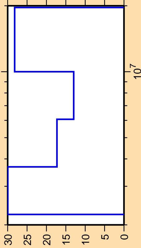
\Delta\sigma/\sigma vs. E for ^{54}\text{Mn}(n,n\text{cont.})
