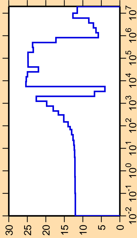
\Delta\sigma/\sigma vs. E for ^{54}\text{Mn}(n,\text{el.})
