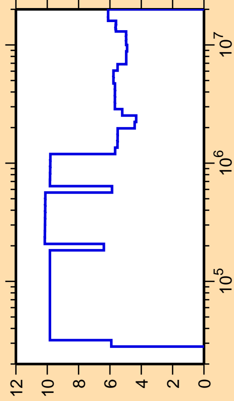
\Delta\sigma/\sigma vs. E for ^{55}\text{Mn}(n,\text{nonel.})
