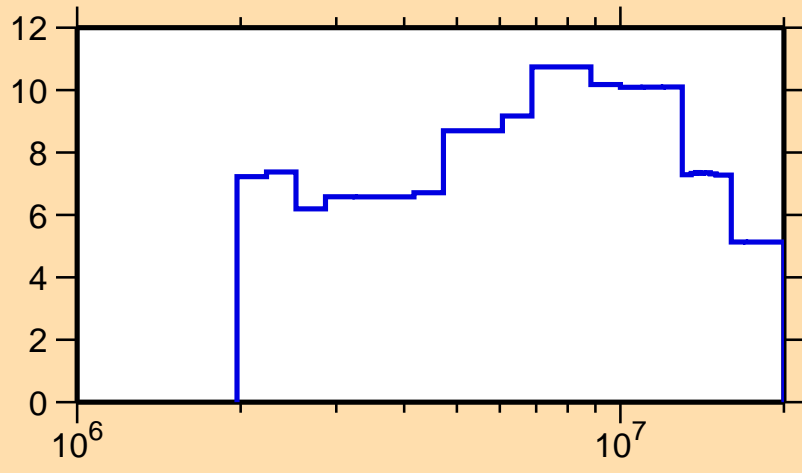
\Delta\sigma/\sigma vs. E for ^{55}\text{Mn}(n,el.)
