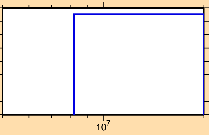
\sigma vs. E for ^{55}\text{Mn}(n,2np)
