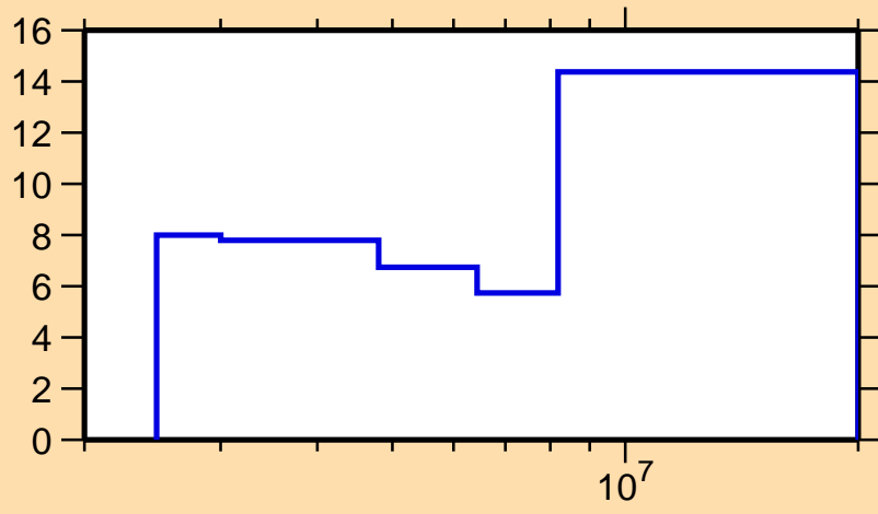
\Delta\sigma/\sigma vs. E for ^{55}\text{Mn}(n,n\text{cont.})
