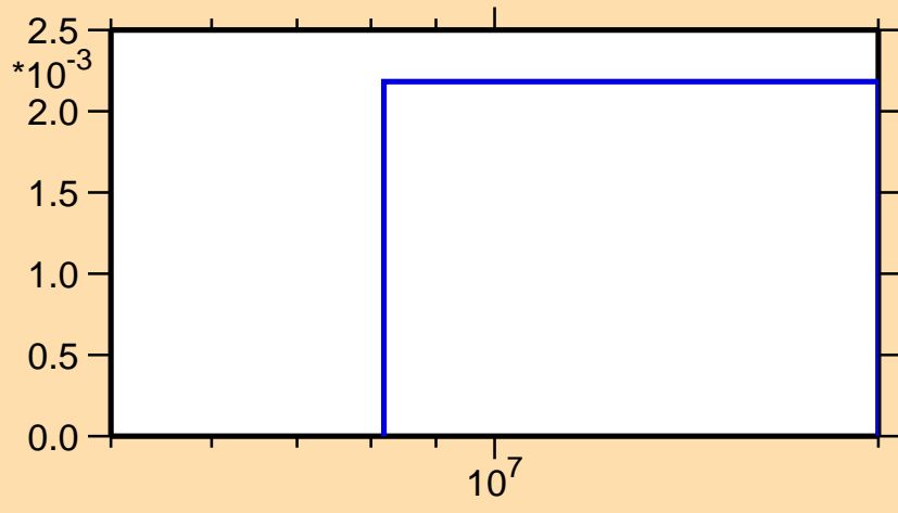
\sigma vs. E for ^{55}\text{Mn}(n,n\alpha)
