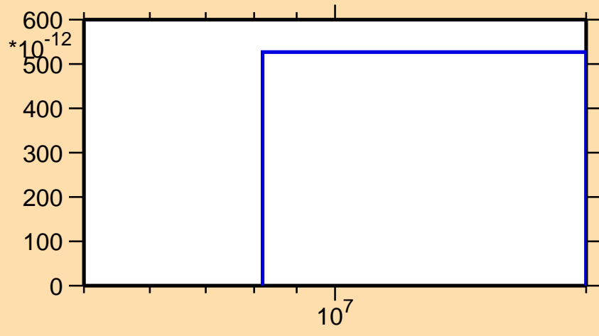
\sigma vs. E for ^{56}\text{Mn}(n,nt)
