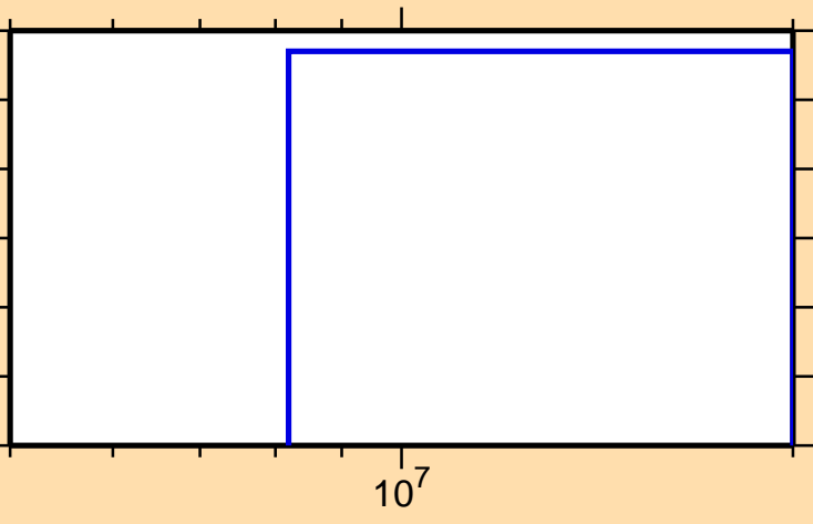
\sigma vs. E for ^{56}\text{Mn}(n,\text{He3})
