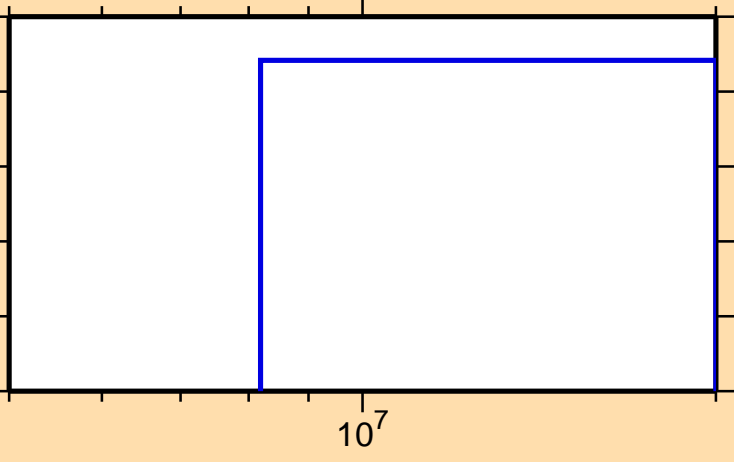
\sigma vs. E for ^{56}\text{Mn}(n,3n)
