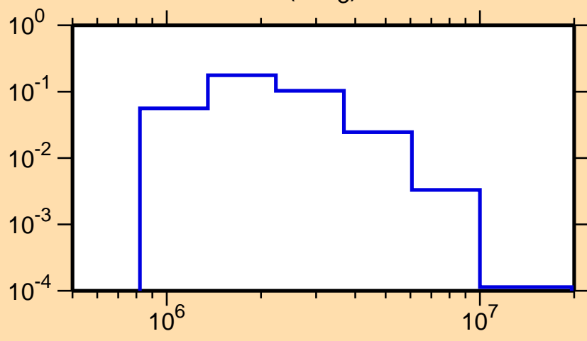
\sigma vs. E for ^{57}\text{Mn}(n,n_3)
