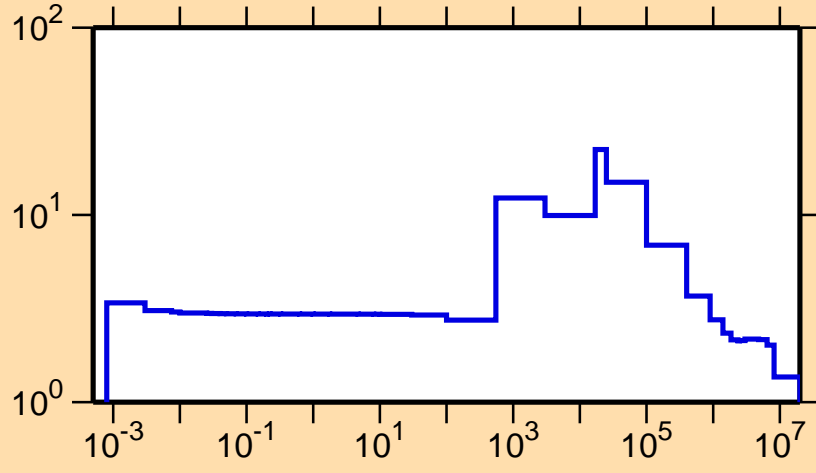
\sigma vs. E for ^{57}\text{Mn}(n,\text{el.})
