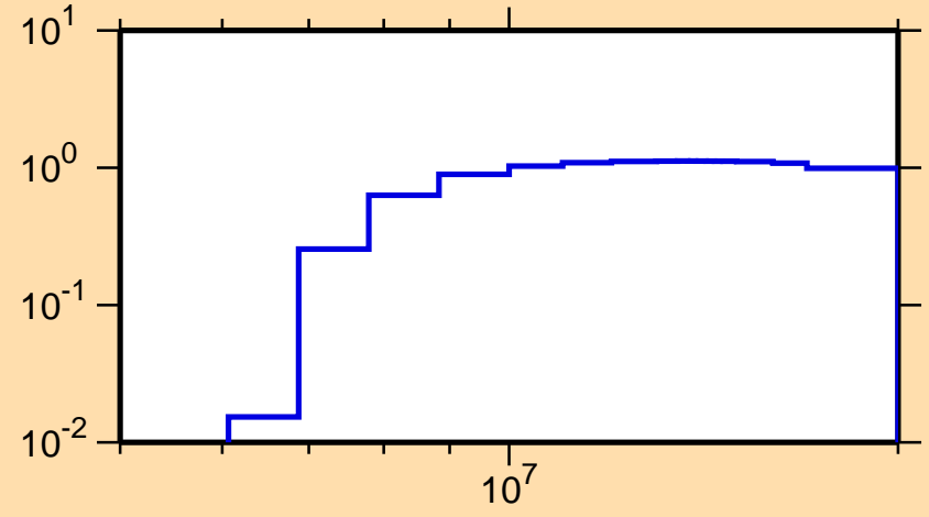
\sigma vs. E for ^{58}\text{Mn}(n,2n)
