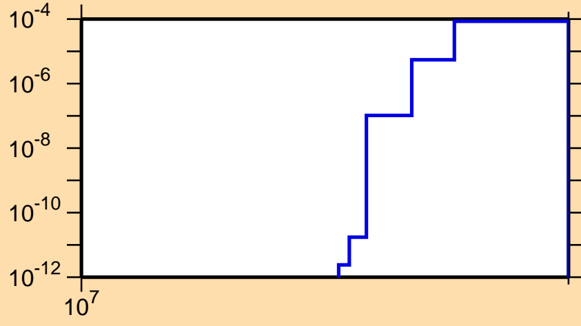
\sigma vs. E for ^{58}\text{Mn}(n,\text{nd})
