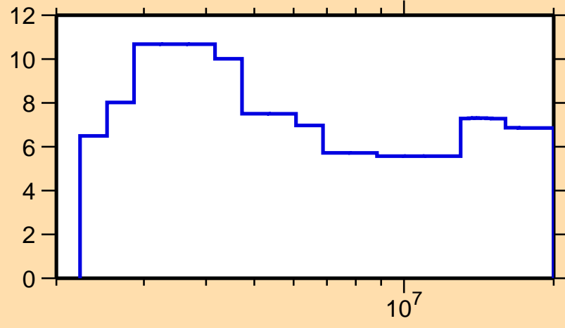
\Delta\sigma/\sigma vs. E for ^{58}\text{Mn}(n,n\text{inel.})
