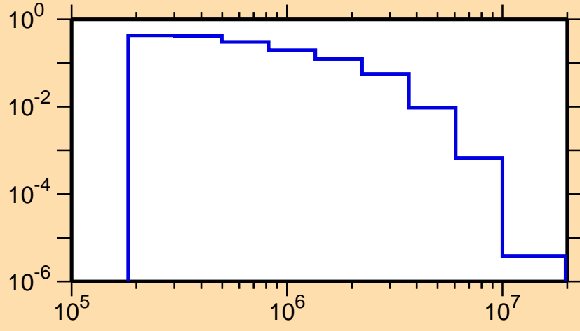
\sigma vs. E for ^{58}\text{Mn}(n,n_4)
