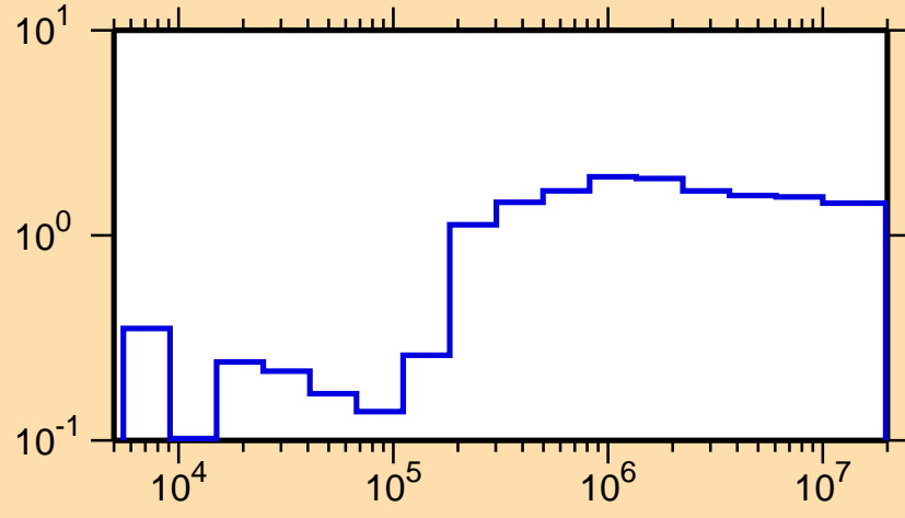
\sigma vs. E for ^{58}\text{Mn}(n,\text{nonel.})
