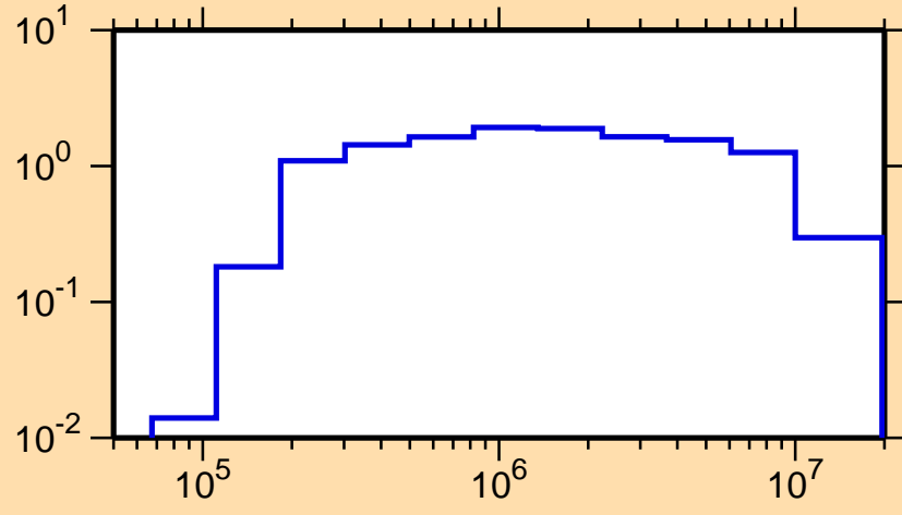
\sigma vs. E for ^{58}\text{Mn}(n,\text{inel.})
