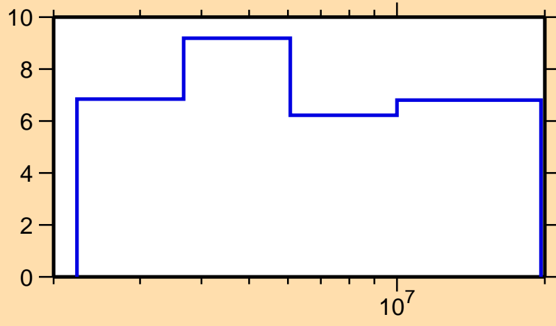
\Delta\sigma/\sigma vs. E for ^{58}\text{Mn}(n,n\text{inel.})
