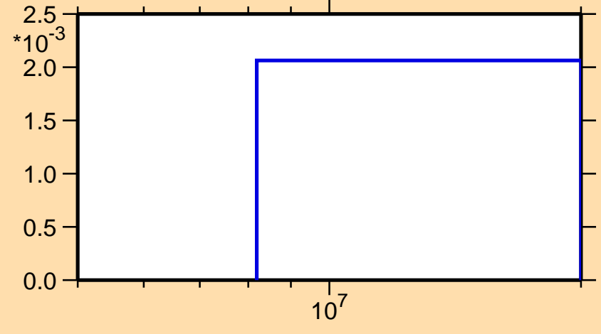
\sigma vs. E for ^{58}\text{Mn}(n,3n)
