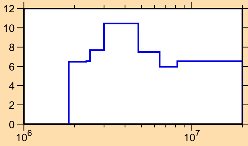
\Delta\sigma/\sigma vs. E for ^{58}\text{Mn}(n,n,\text{nonel.})
