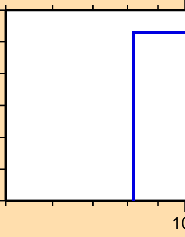
\sigma vs. E for ^{58}\text{Mn}(n,2np)
