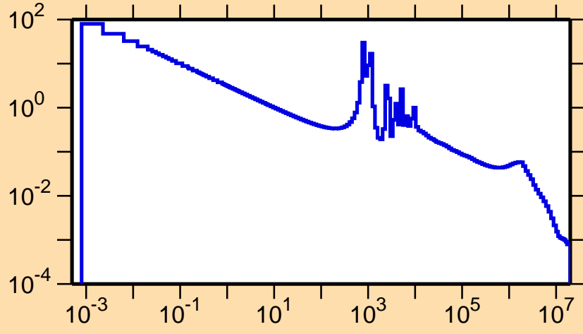
\sigma vs. E for ^{59}\text{Mn}(n,\gamma)
