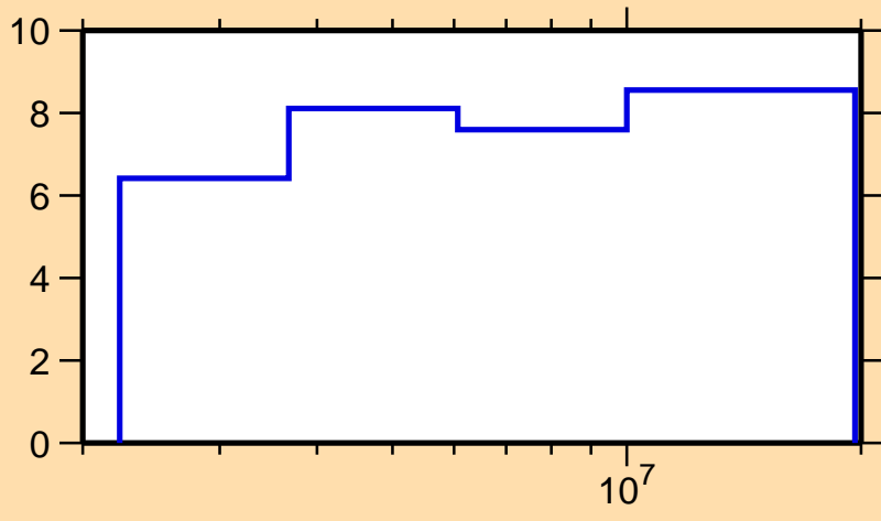
\Delta\sigma/\sigma vs. E for ^{59}\text{Mn}(n,n\text{inel.})
