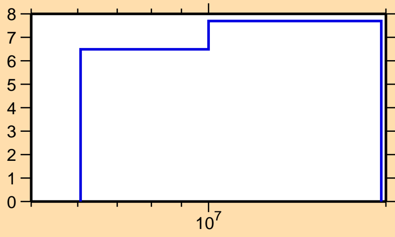
\Delta\sigma/\sigma vs. E for ^{59}\text{Mn}(n,el.)
