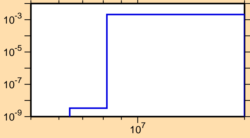
\sigma vs. E for ^{59}\text{Mn}(n,p)
