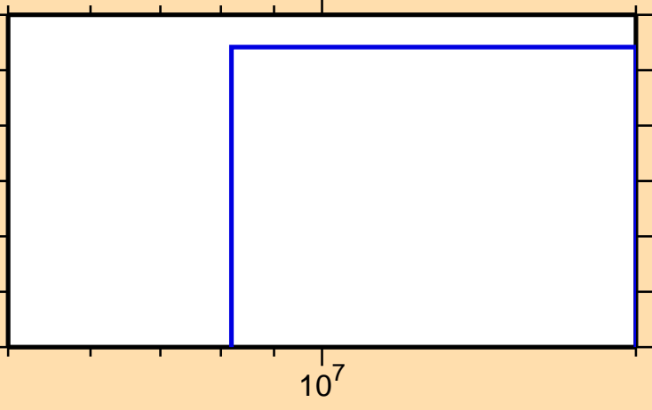
\sigma vs. E for ^{59}\text{Mn}(n,2n\alpha)
