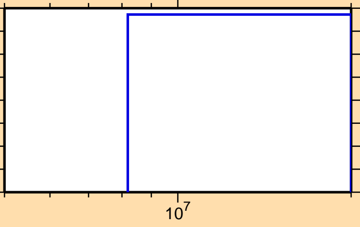
\sigma vs. E for ^{59}\text{Mn}(n,t)
