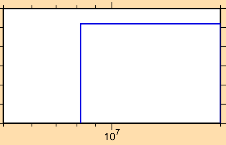
\sigma vs. E for ^{59}\text{Mn}(n,2np)
